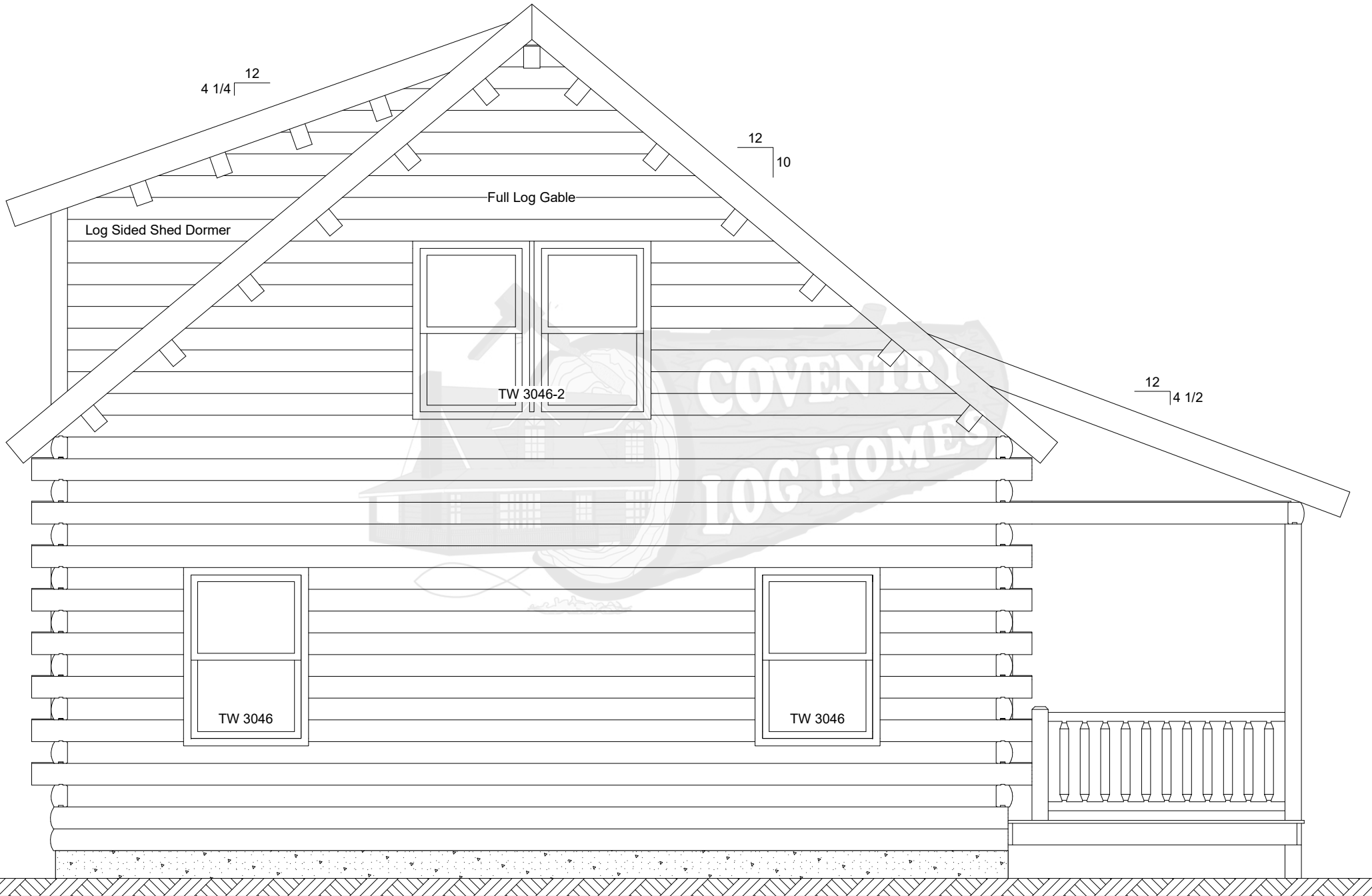
Rear Elevation
