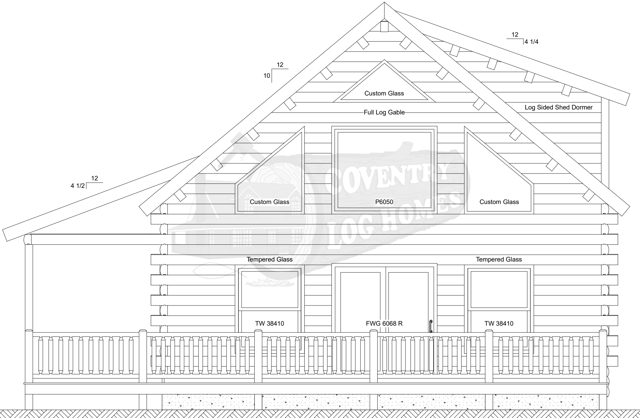
Front Elevation
