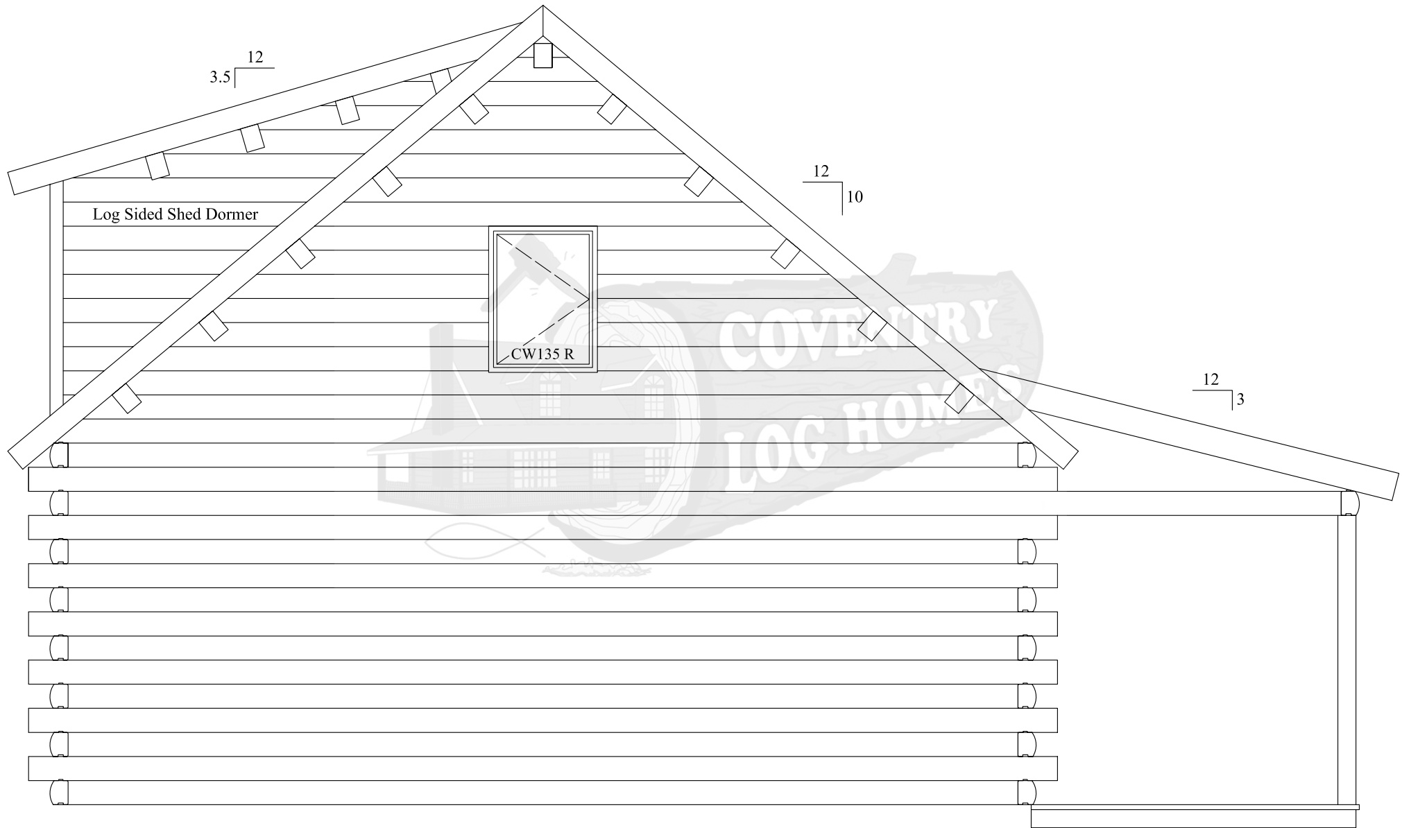
Left Elevation
