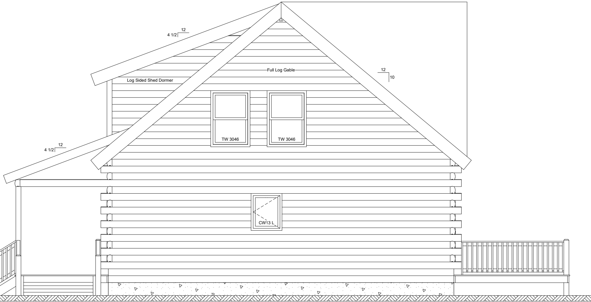
Cascade Right Elevation
