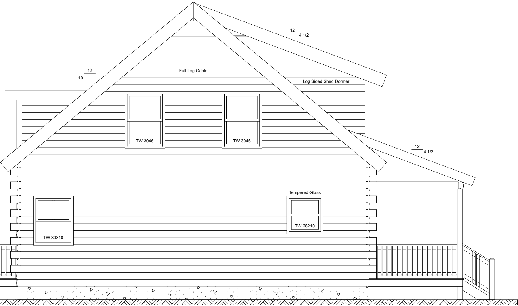
Cascade Left Elevation
