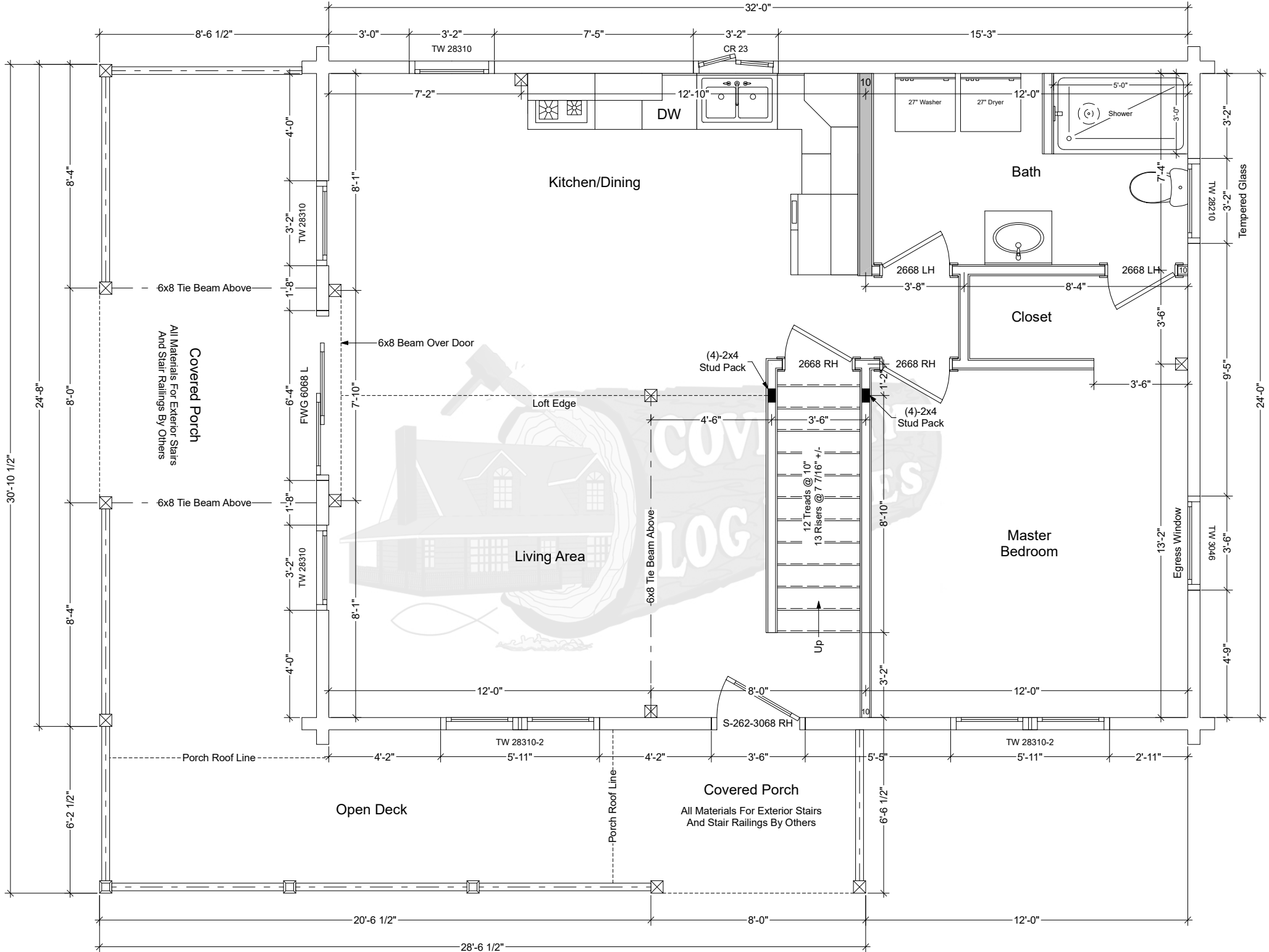
Driftwood First Floor Plan
