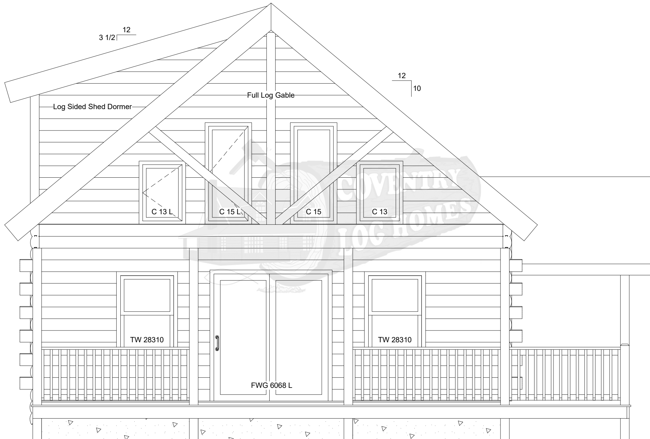
Driftwood Left Elevation
