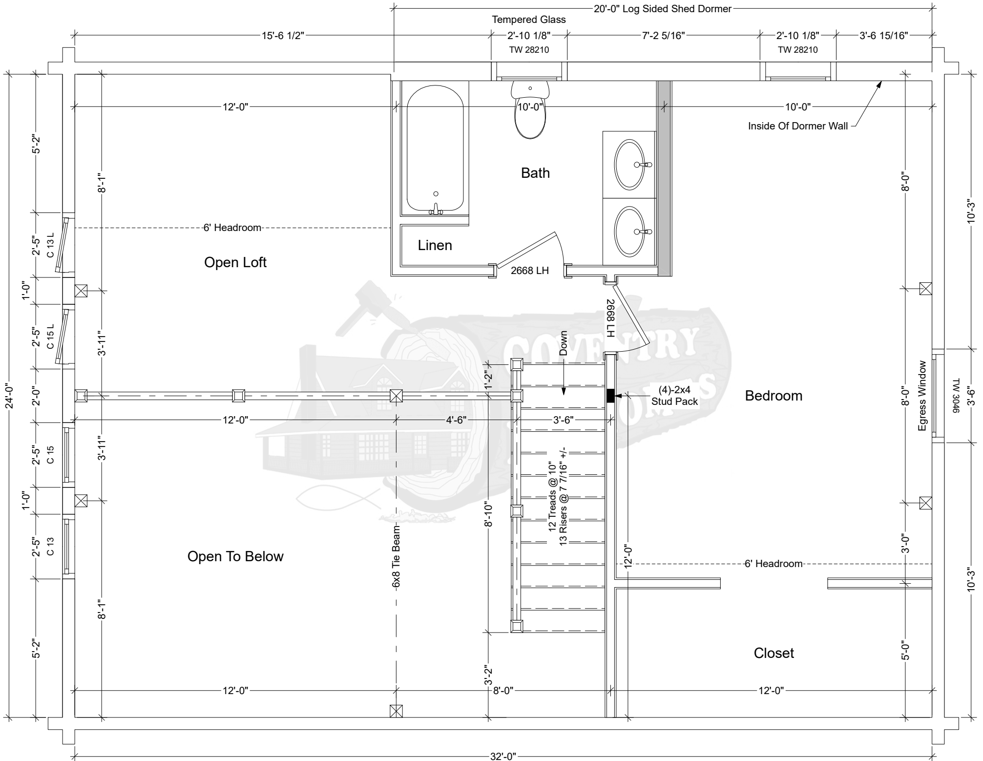
Driftwood Second Floor Plan
