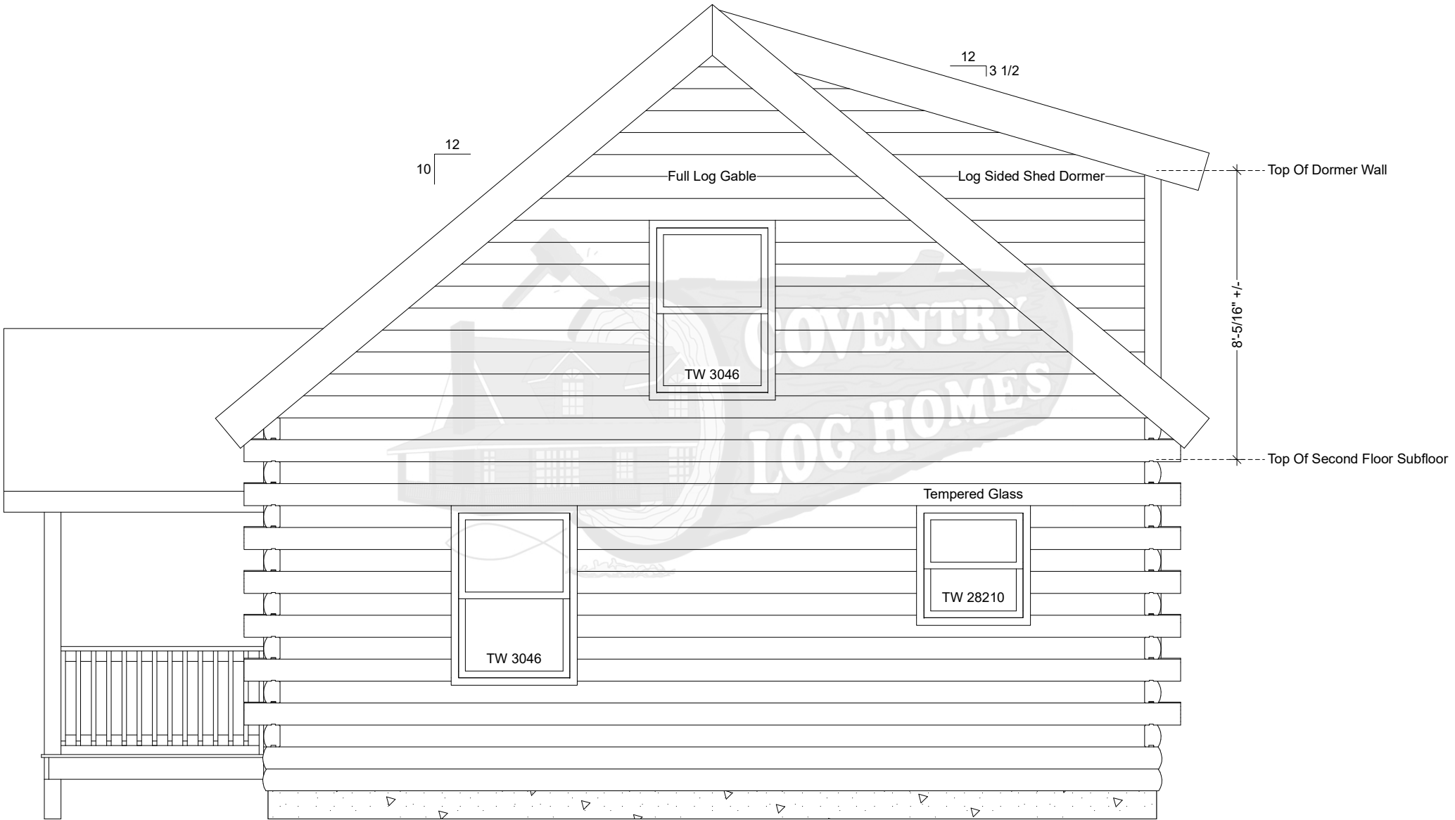
Driftwood Right Elevation
