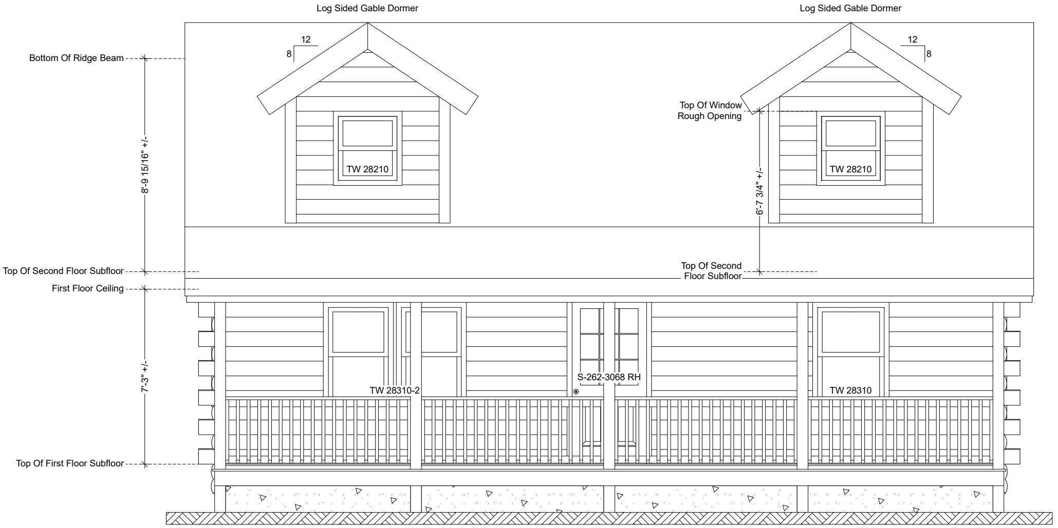
Fairfield Front Elevation
