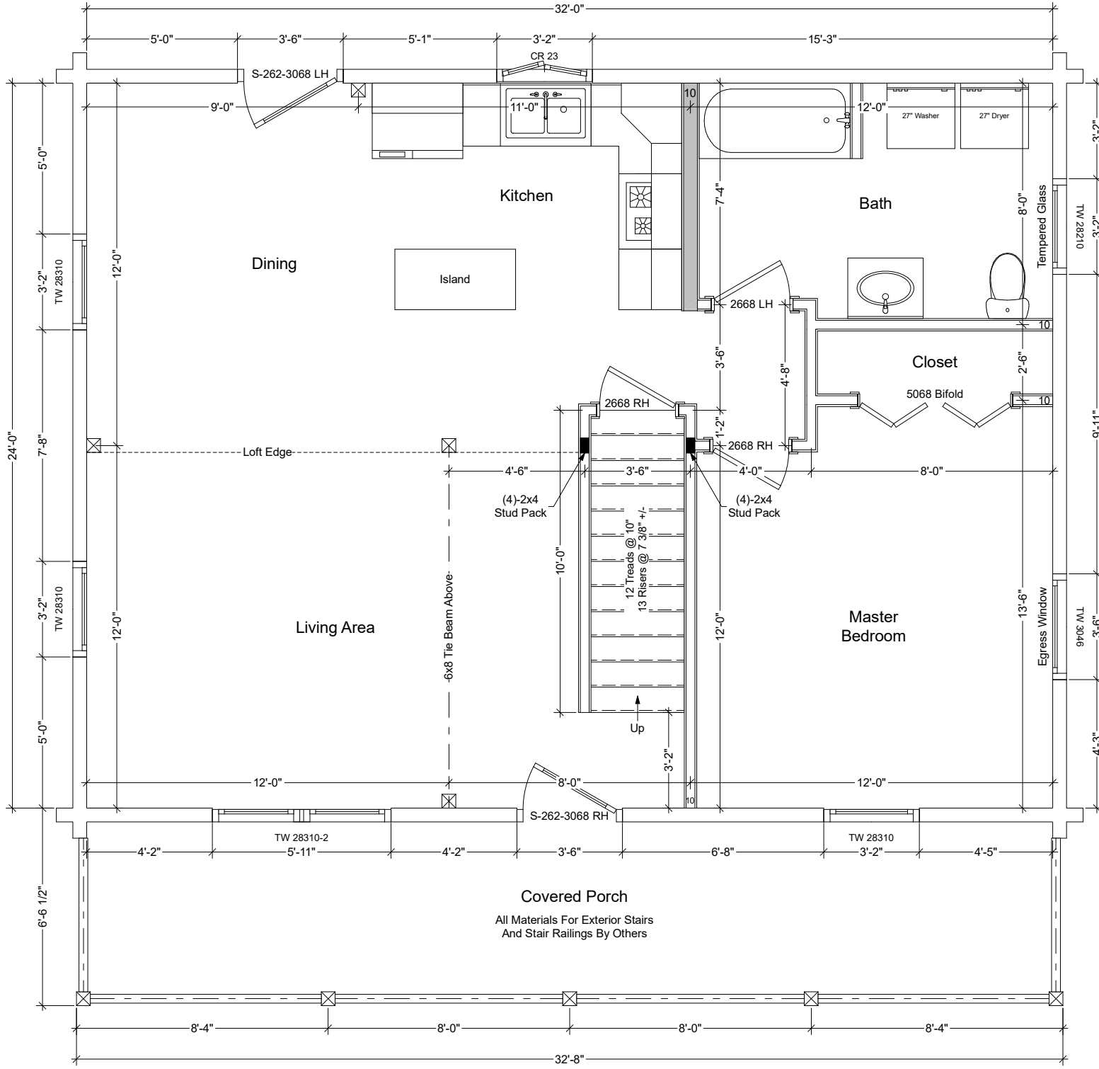
Fairfield First Floor Plan
