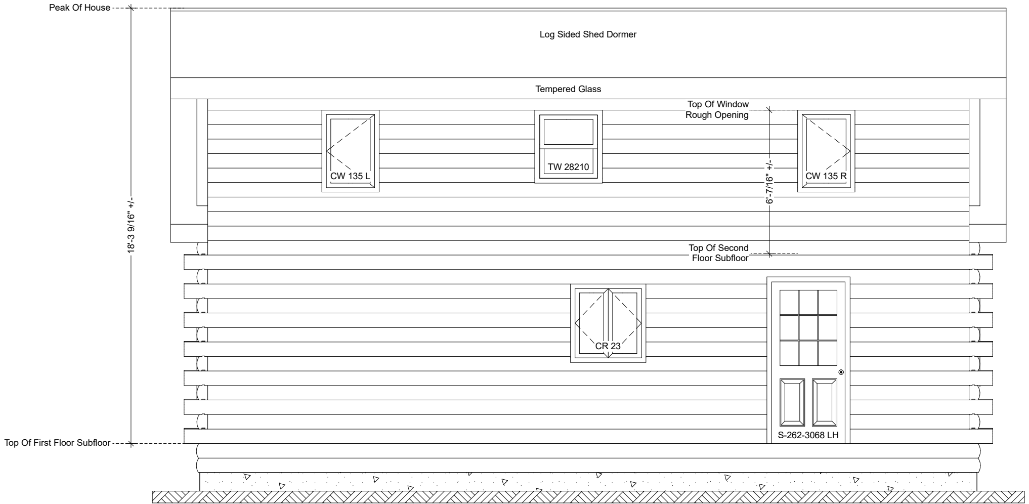
Fairfield Rear Elevation
