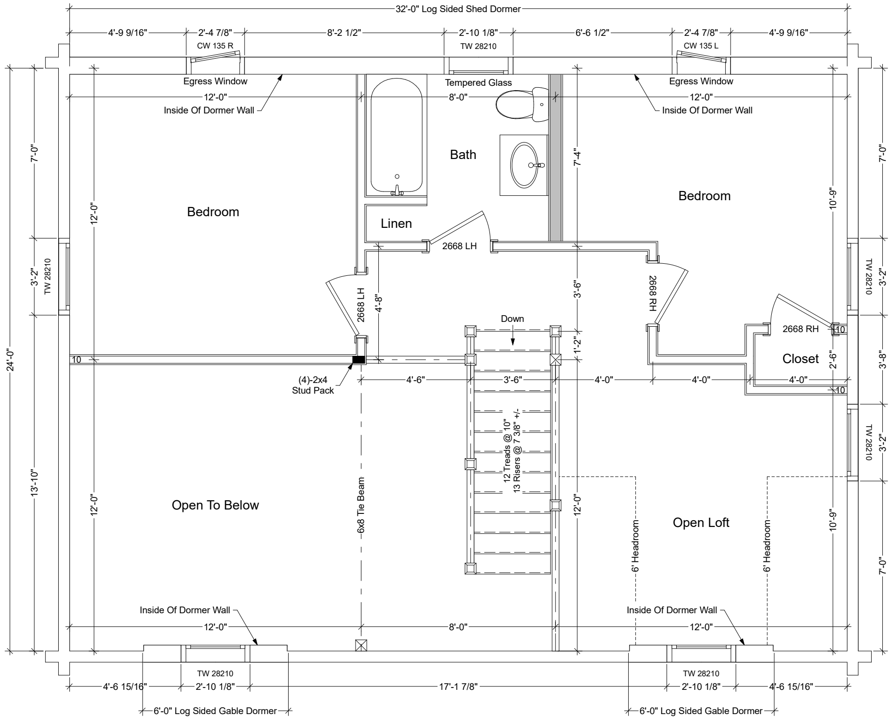
Fairfield Second Floor Plan
