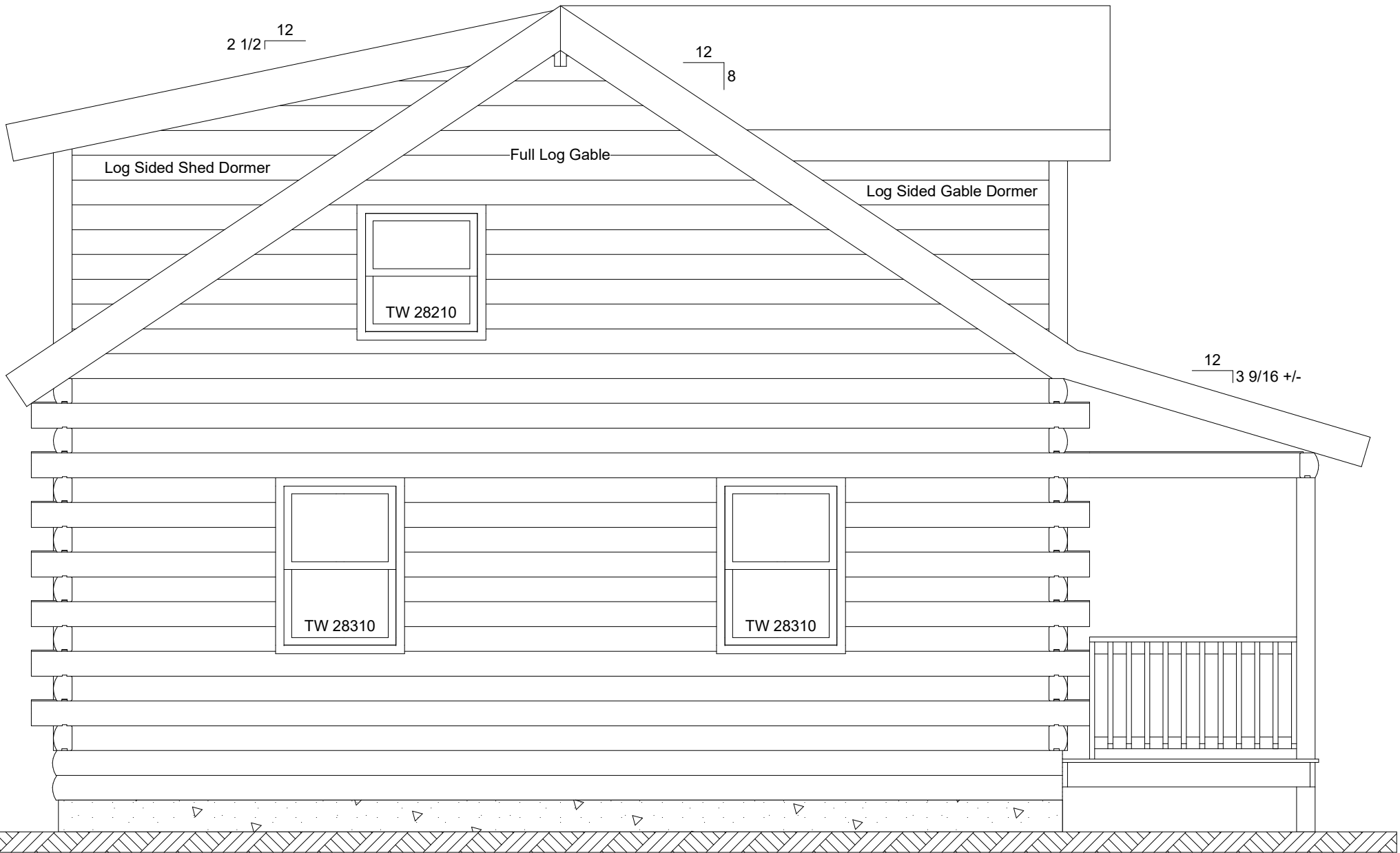
Fairfield Left Elevation
