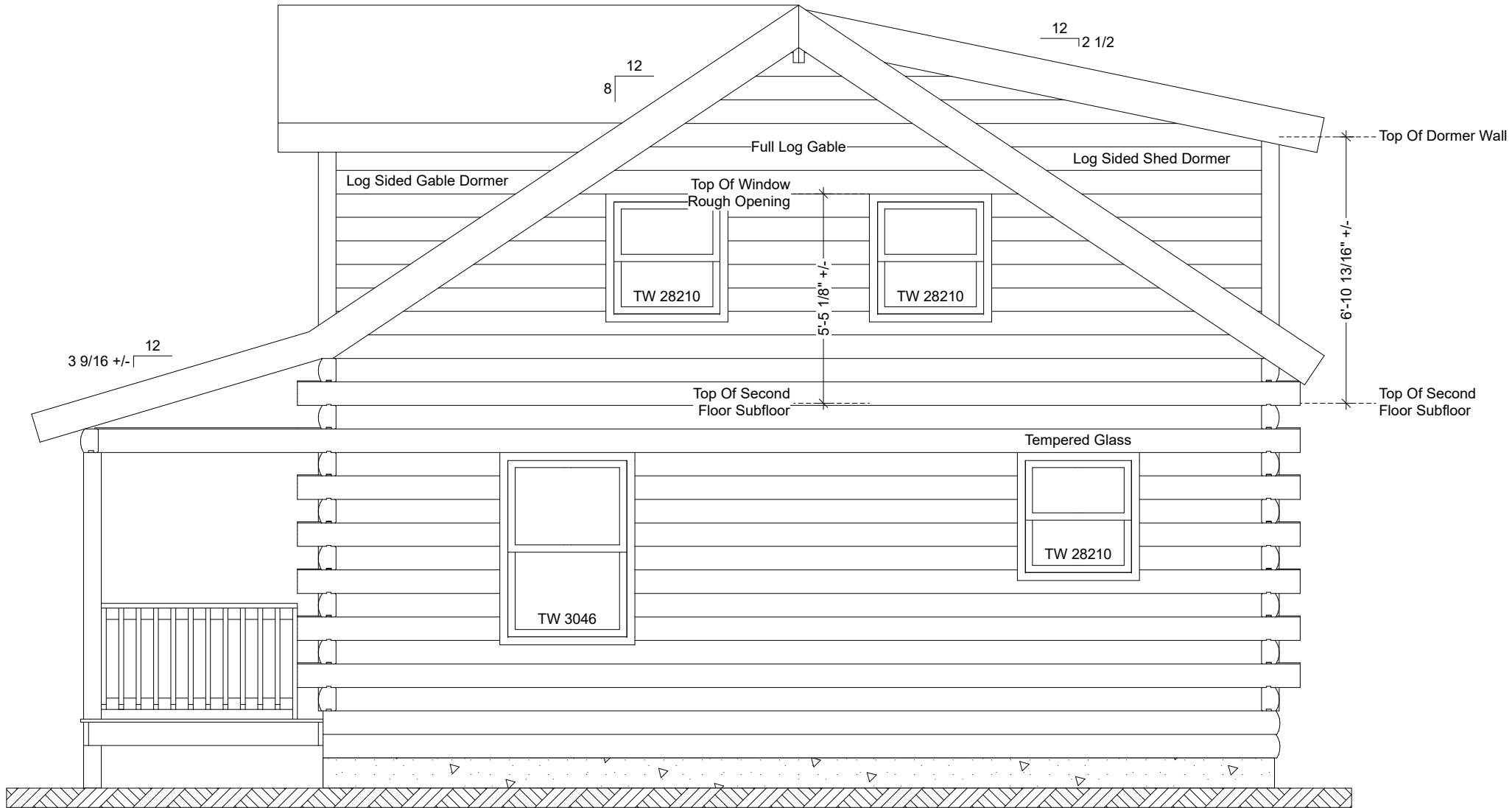
Fairfield Right Elevation
