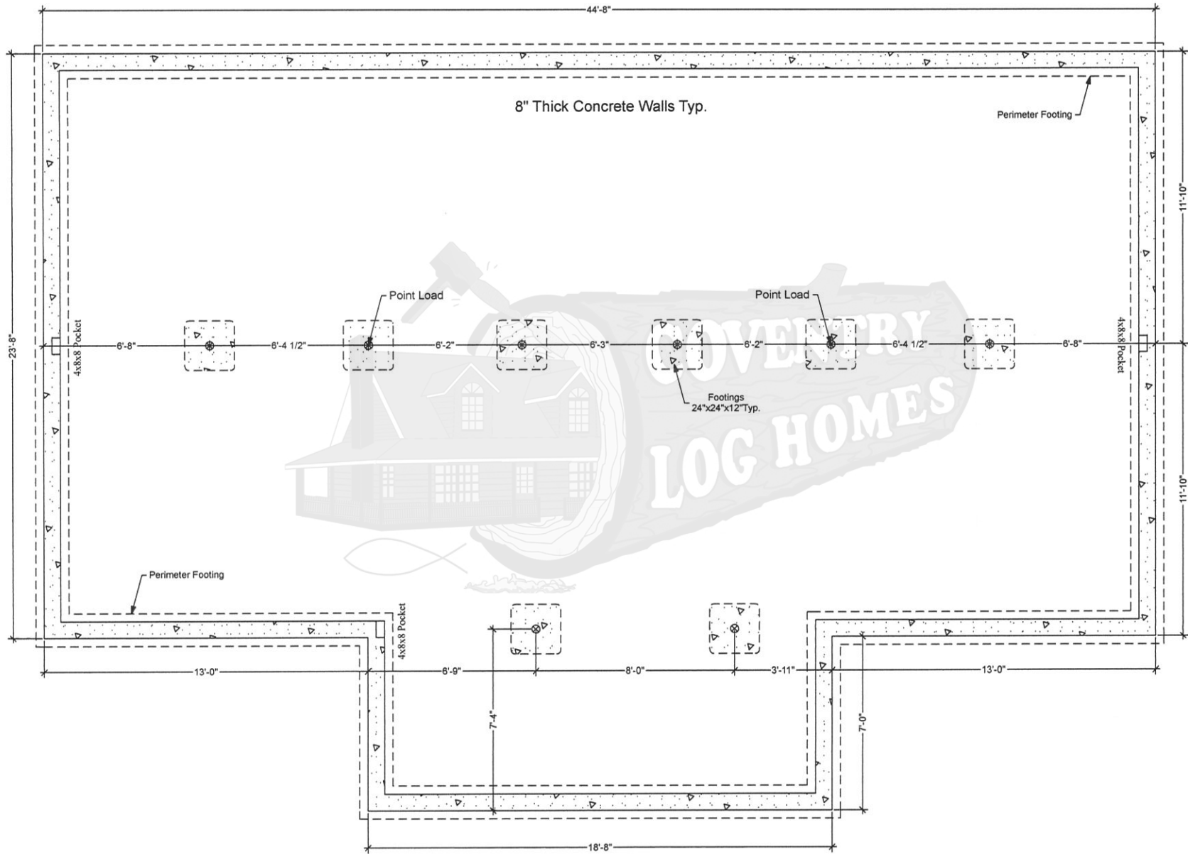
Foundation Plan
