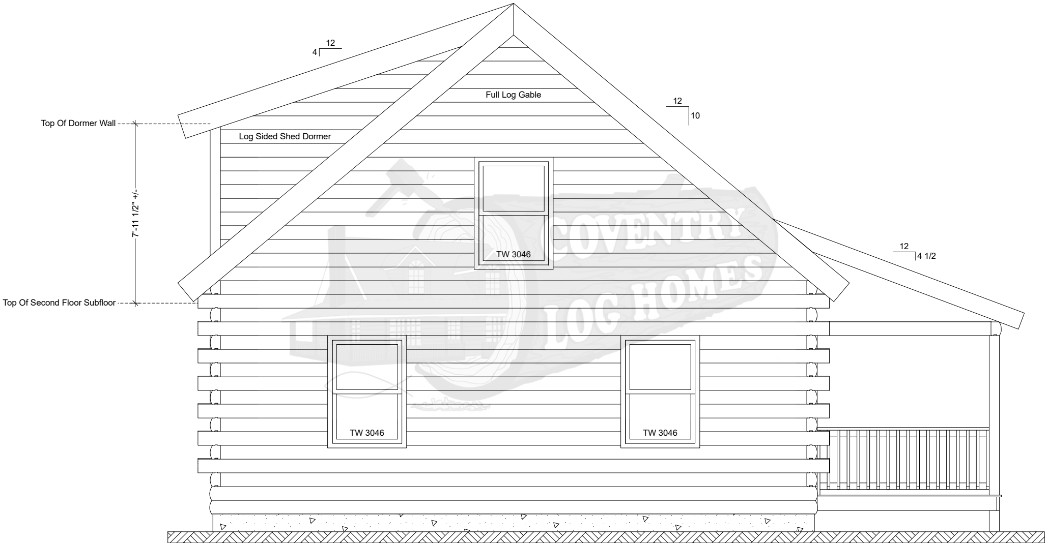
Oak Ridge Rear Elevation
