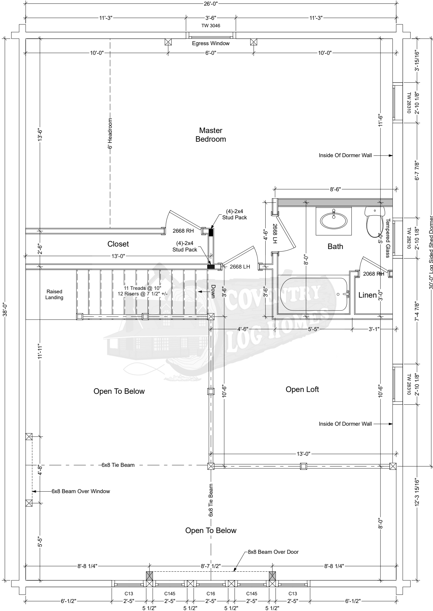
Oak Ridge Second Floor Plan
