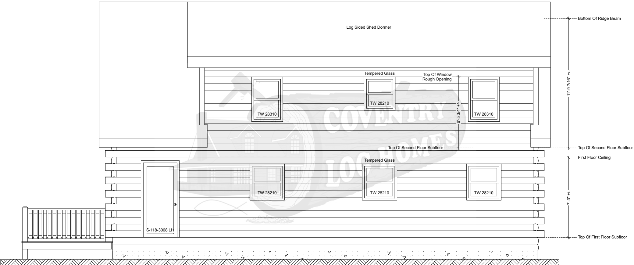
Oak Ridge Right Elevation
