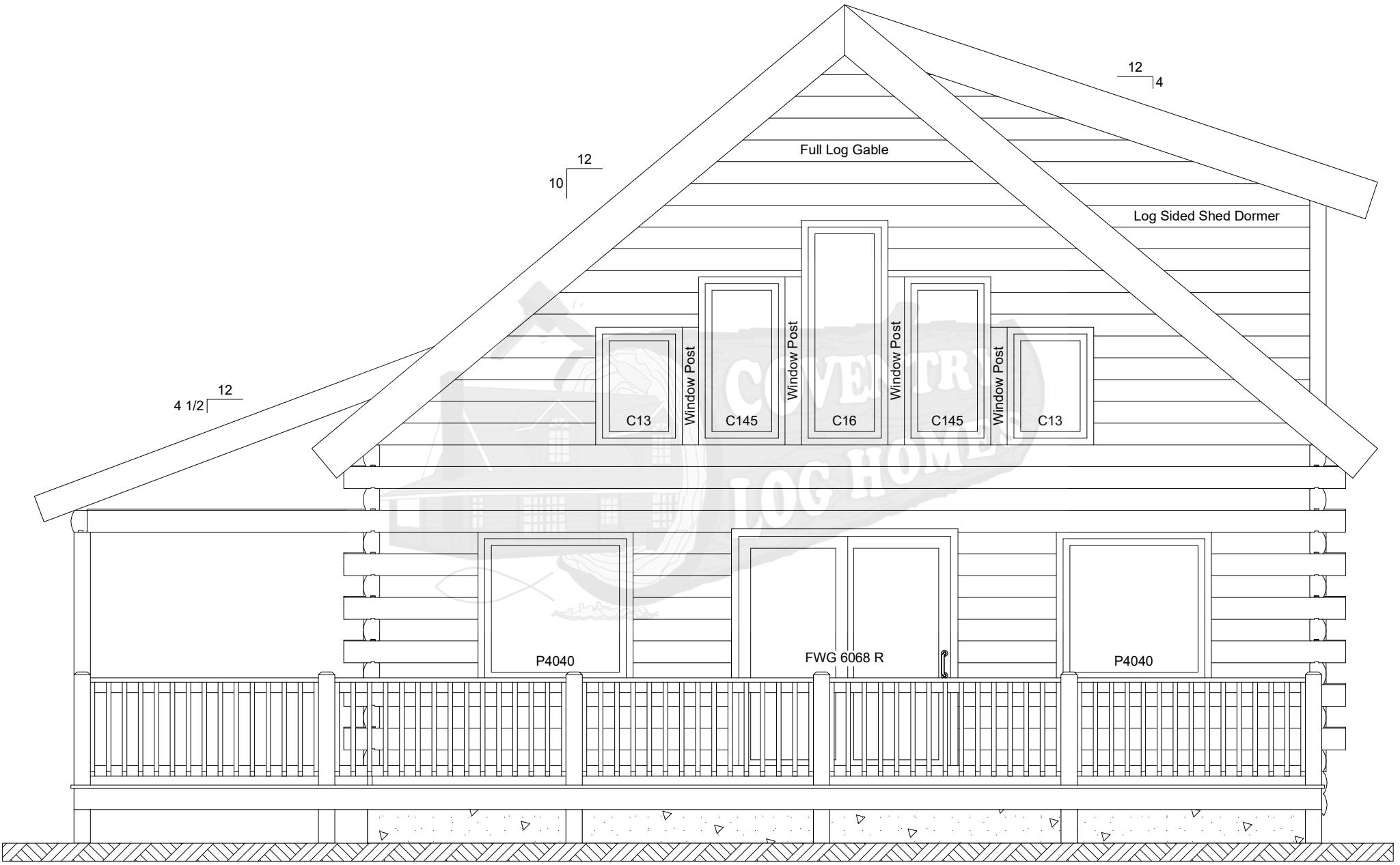
Oak Ridge Front Elevation
