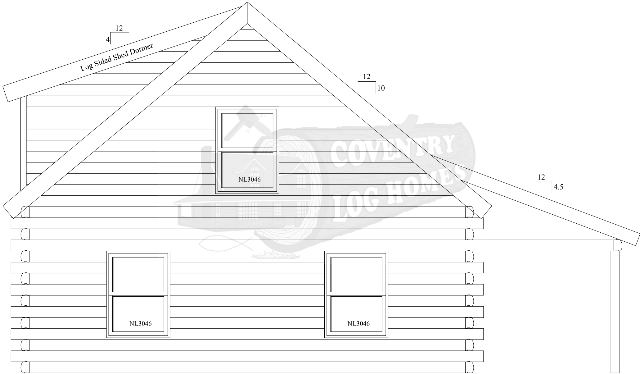
Elevation C
