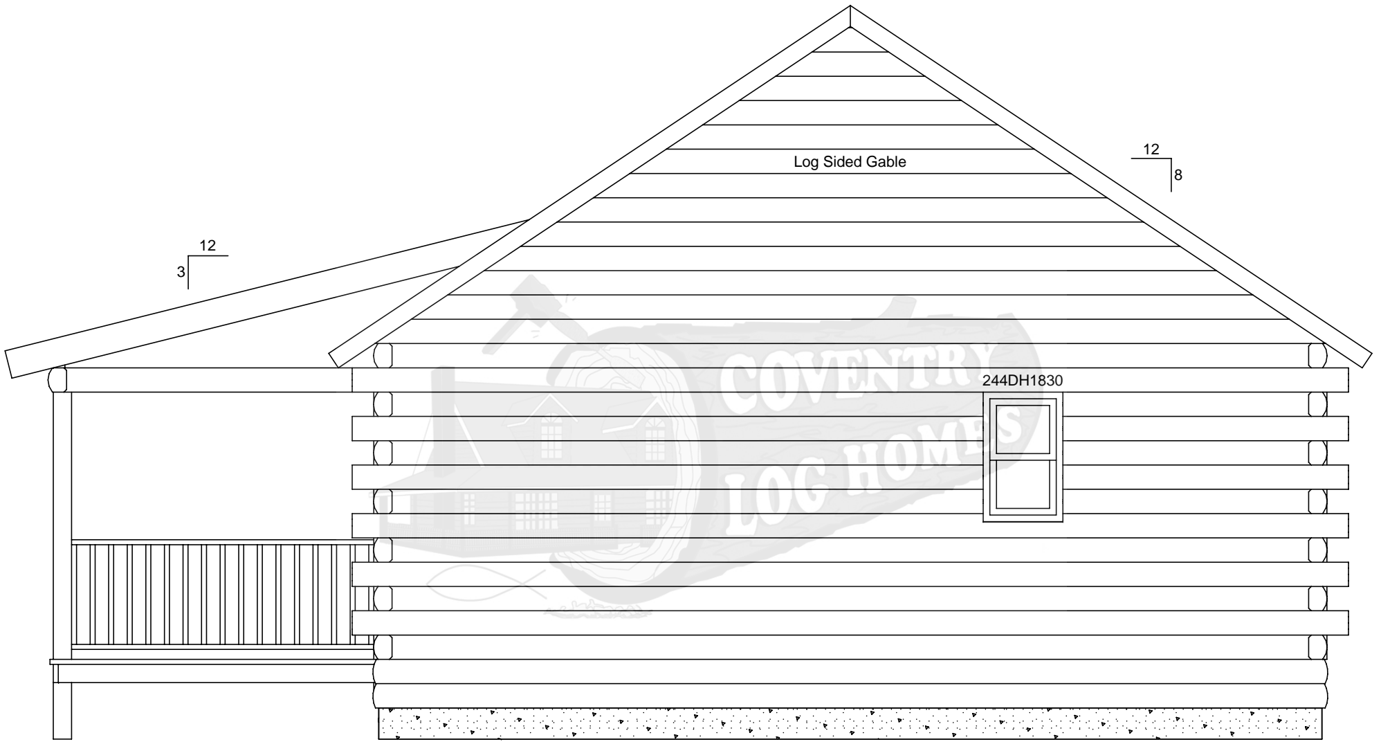
Elevation B Stoney Creek
