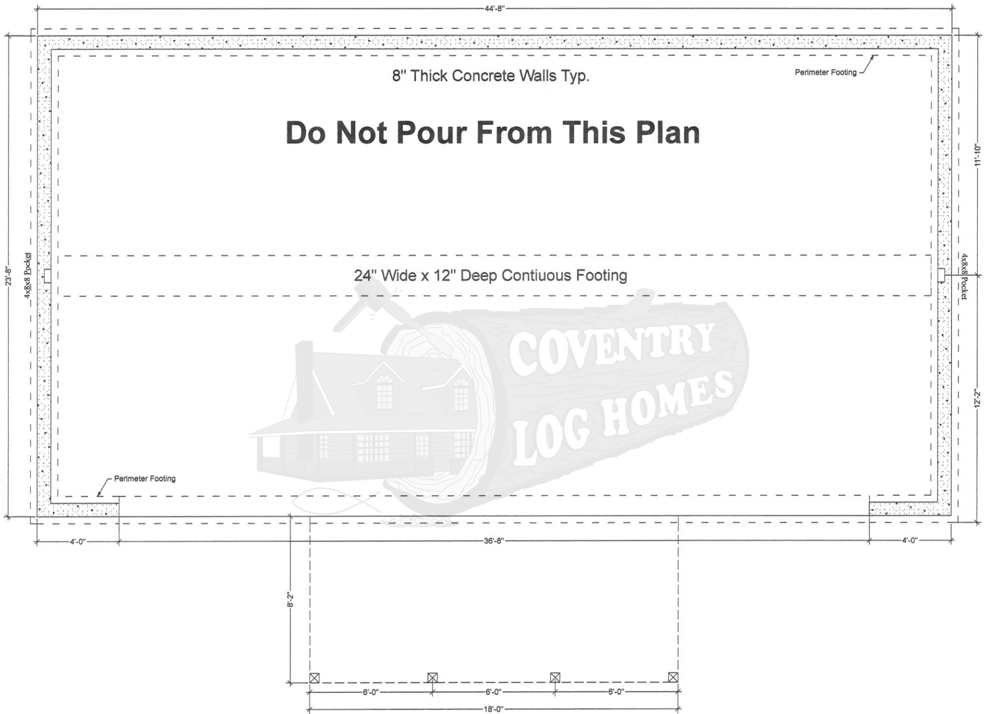
Foundation Plan Stoney Creek
