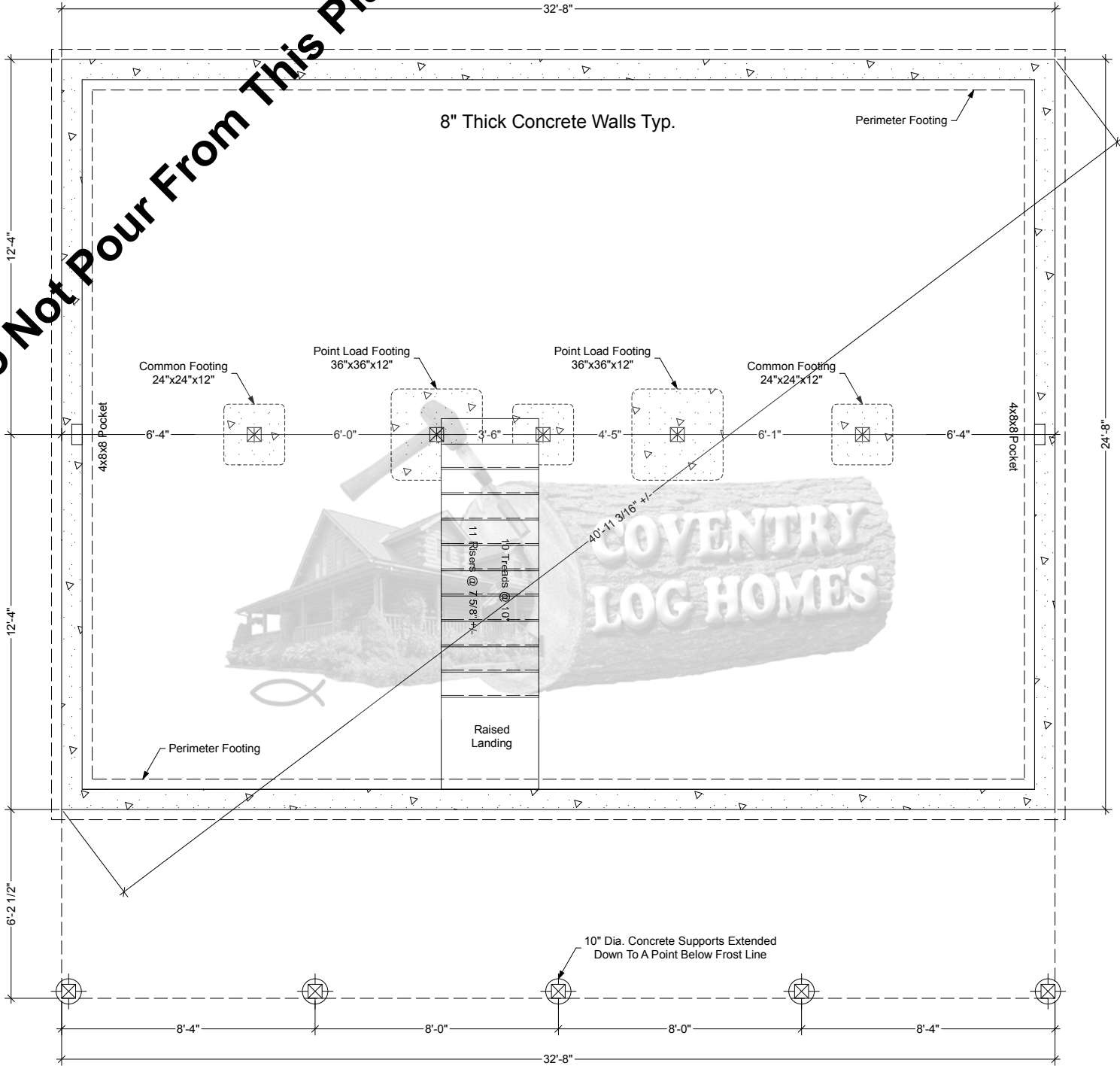
Foundation Plan
