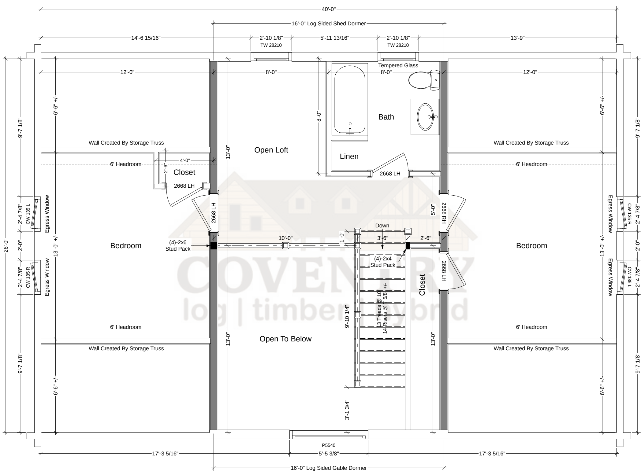
Riverbend Second Floor Plan
