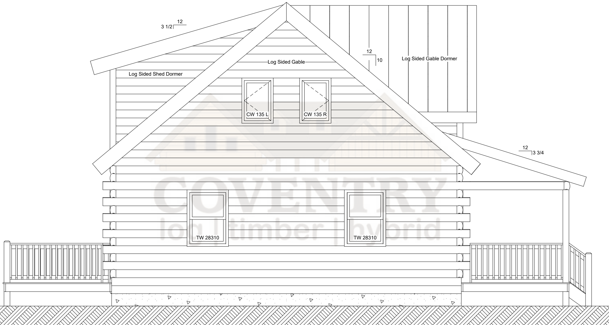
Riverbend Left Elevation
