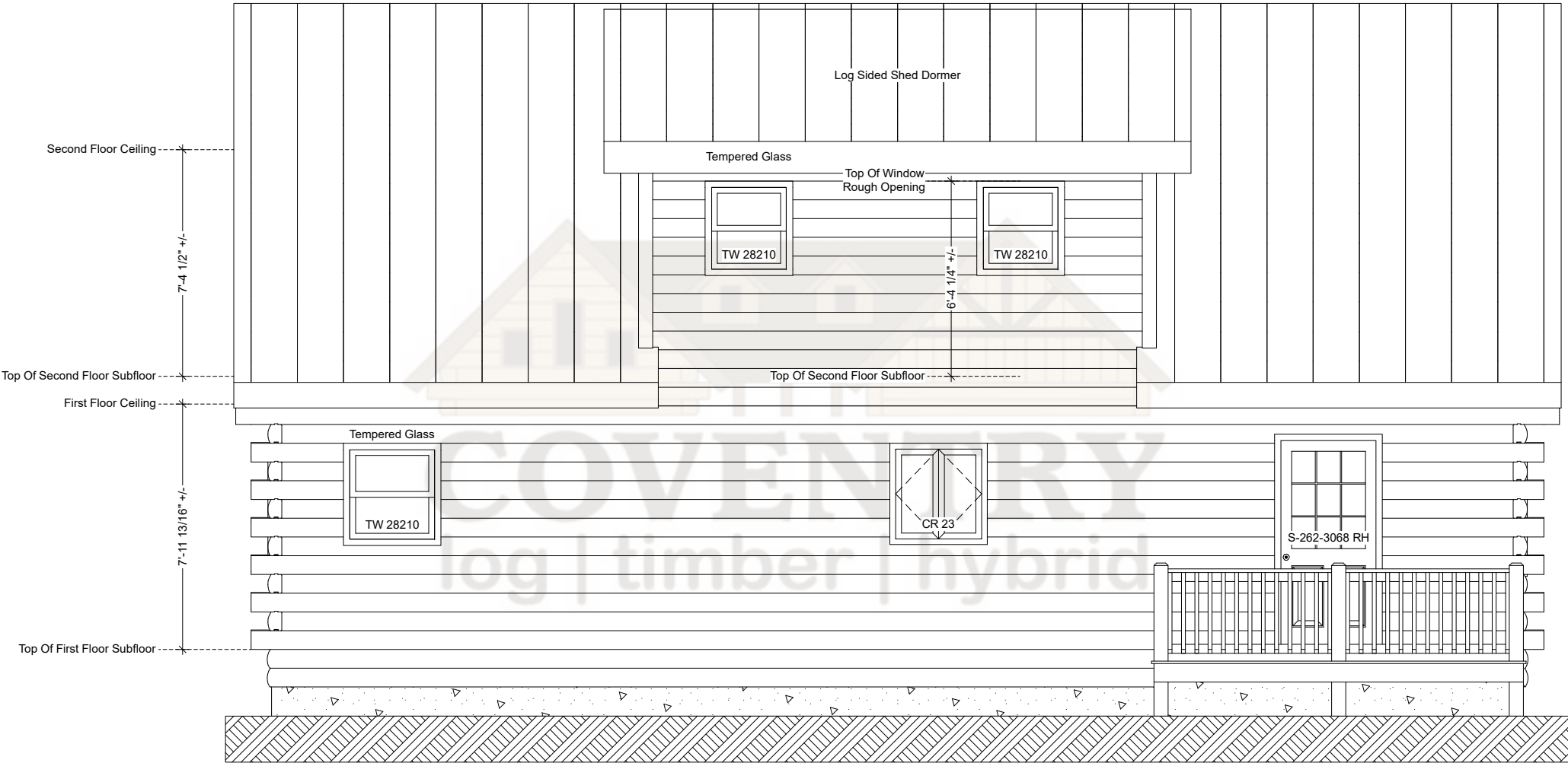
Riverbend Rear Elevation
