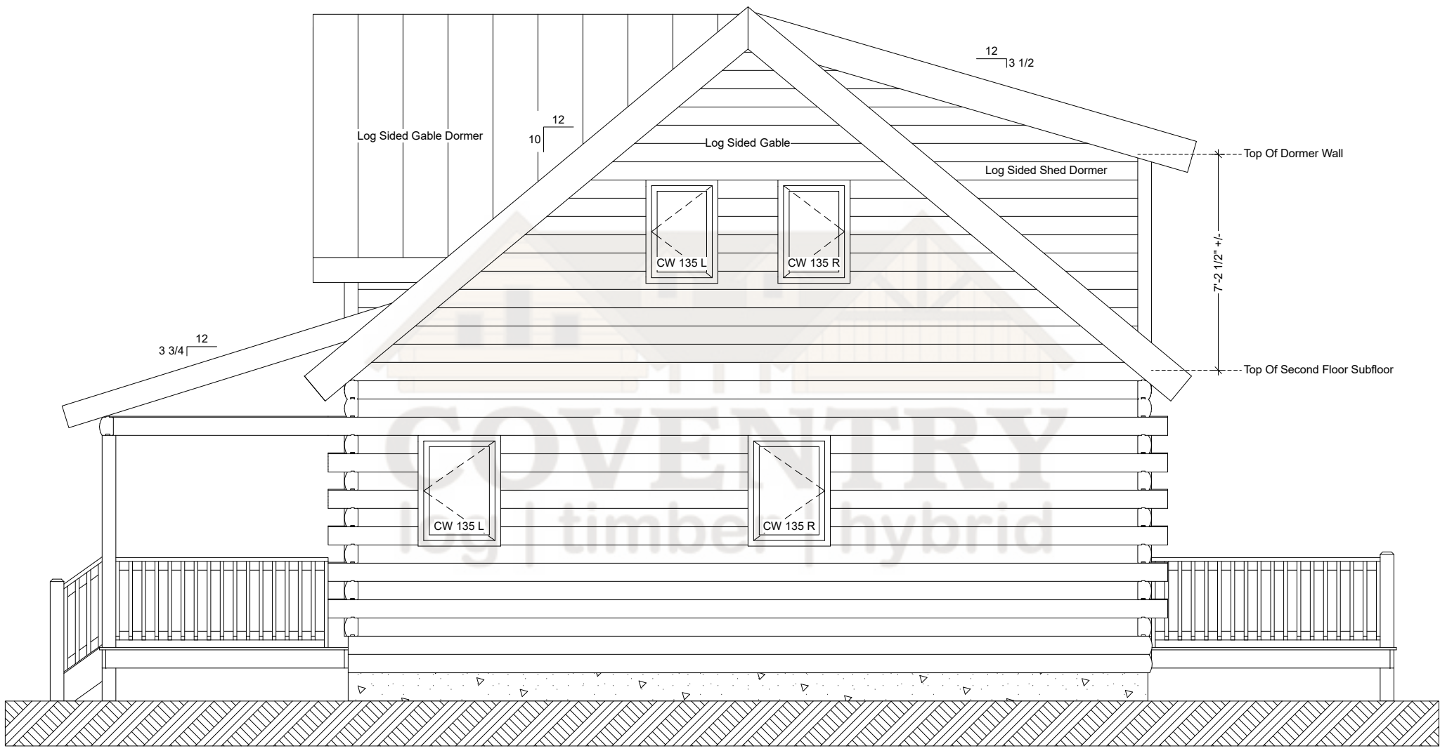
Riverbend Right Elevation
