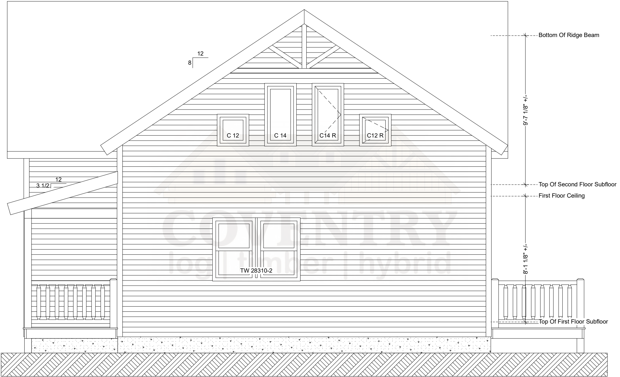
Meredith Right Elevation
