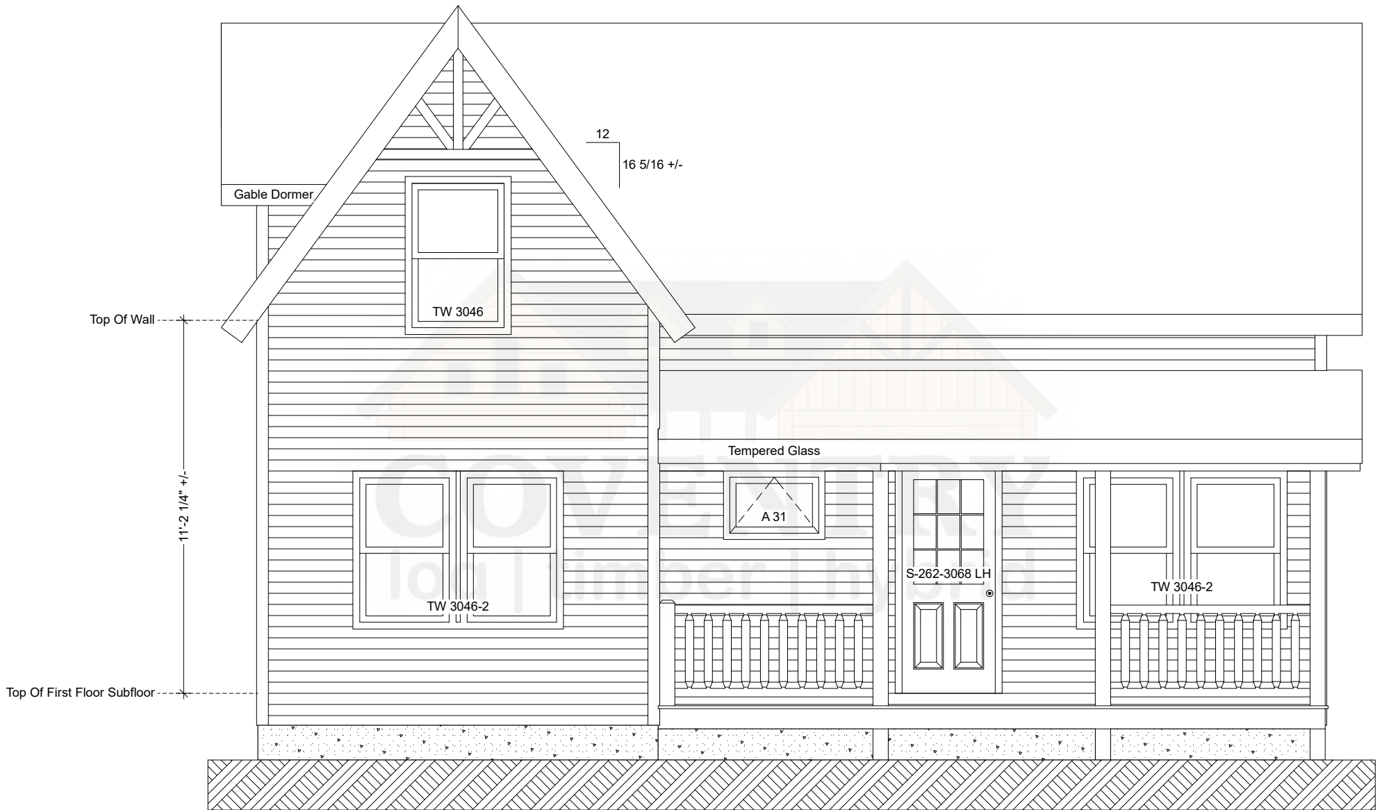
Meredith Front Elevation
