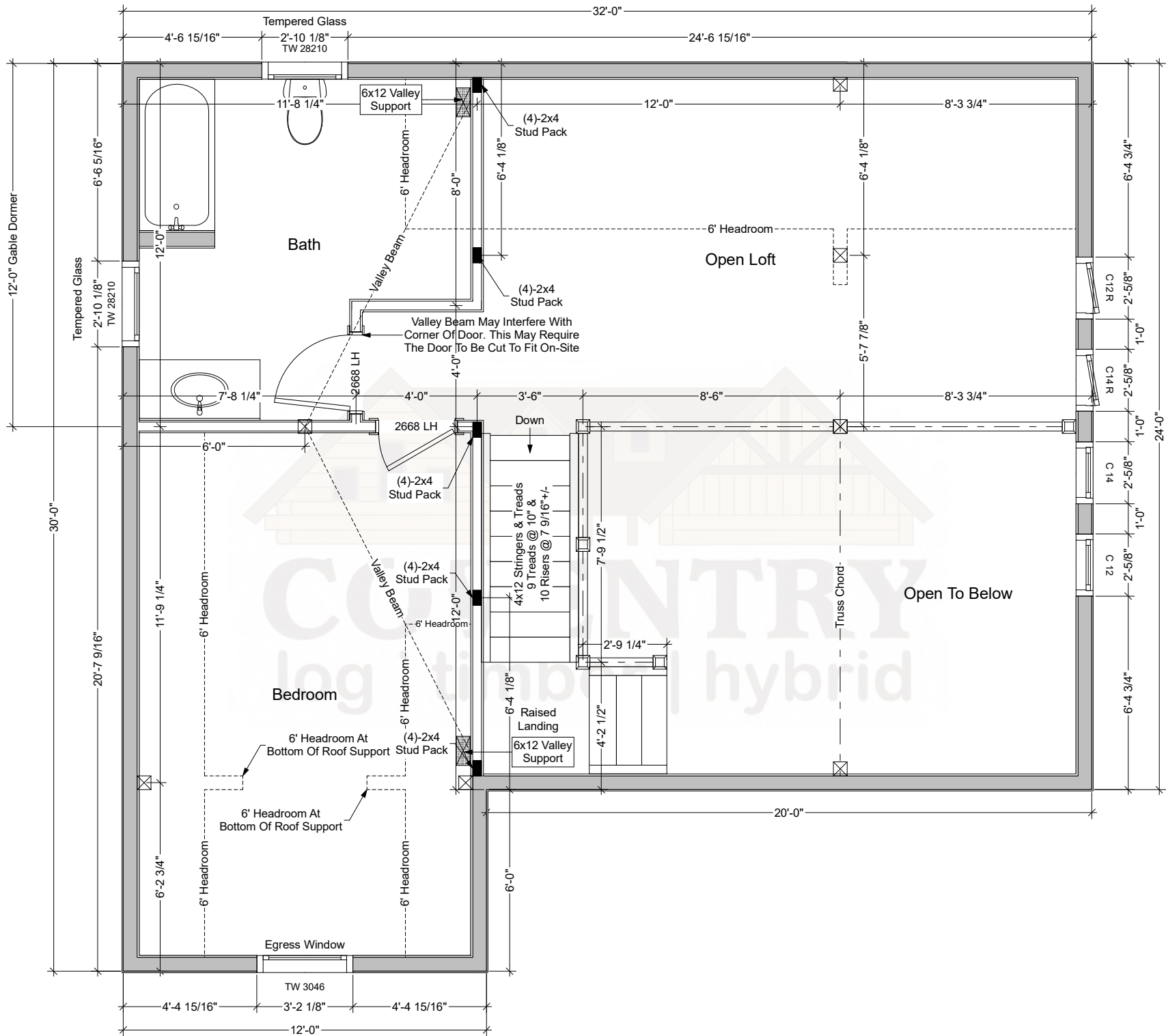
Meredith Second Floor Plan
