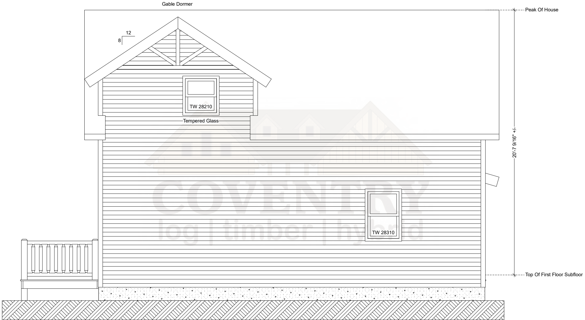
Meredith Left Elevation
