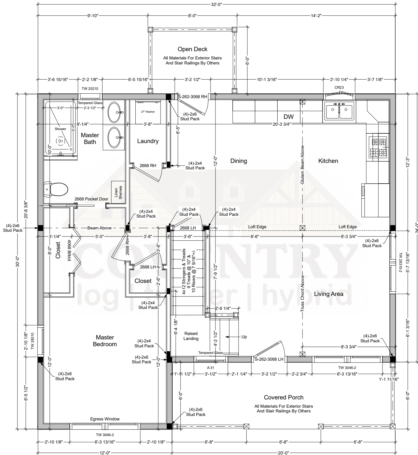
Meredith First Floor Plan
