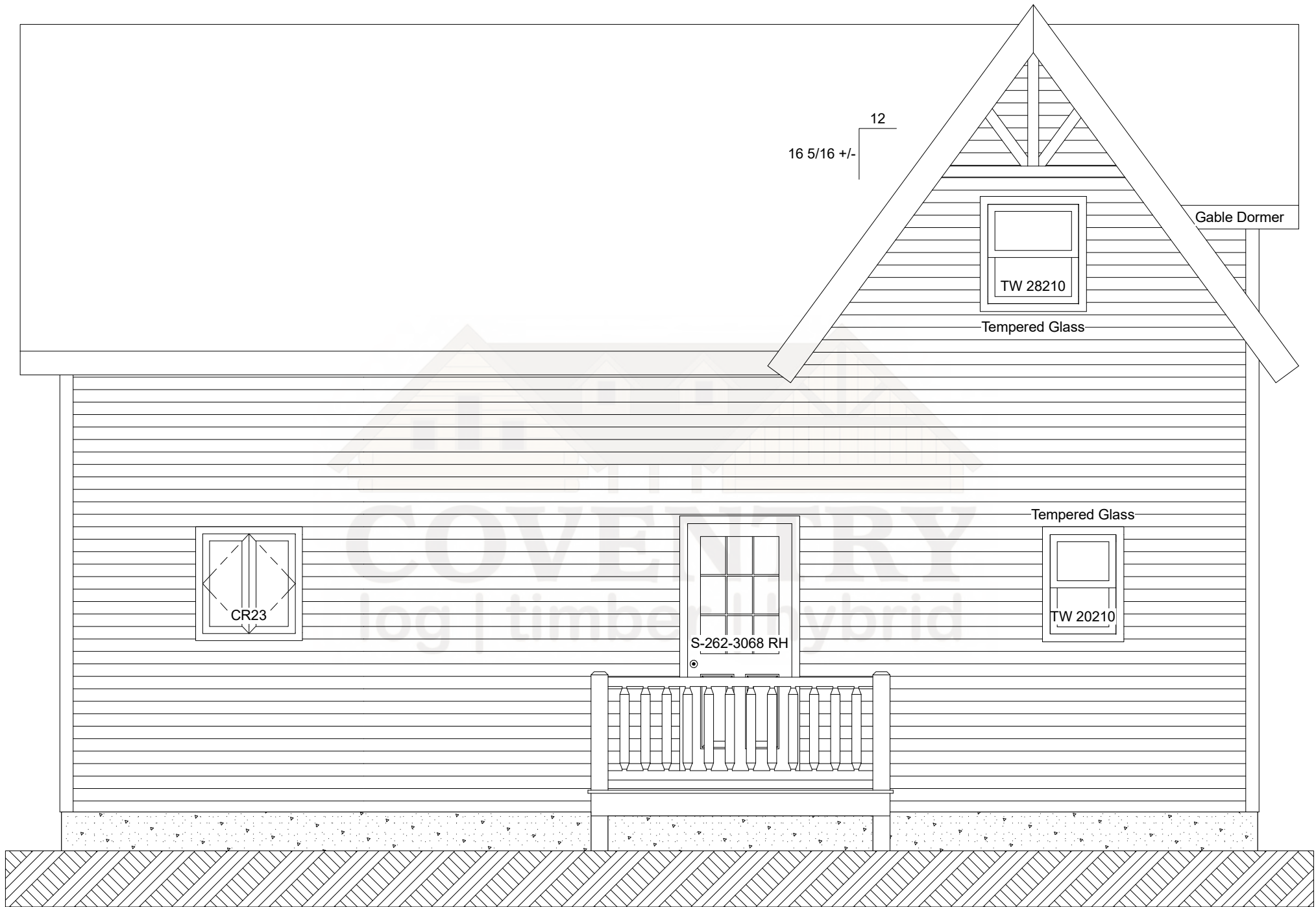
Meredith Rear Elevation
