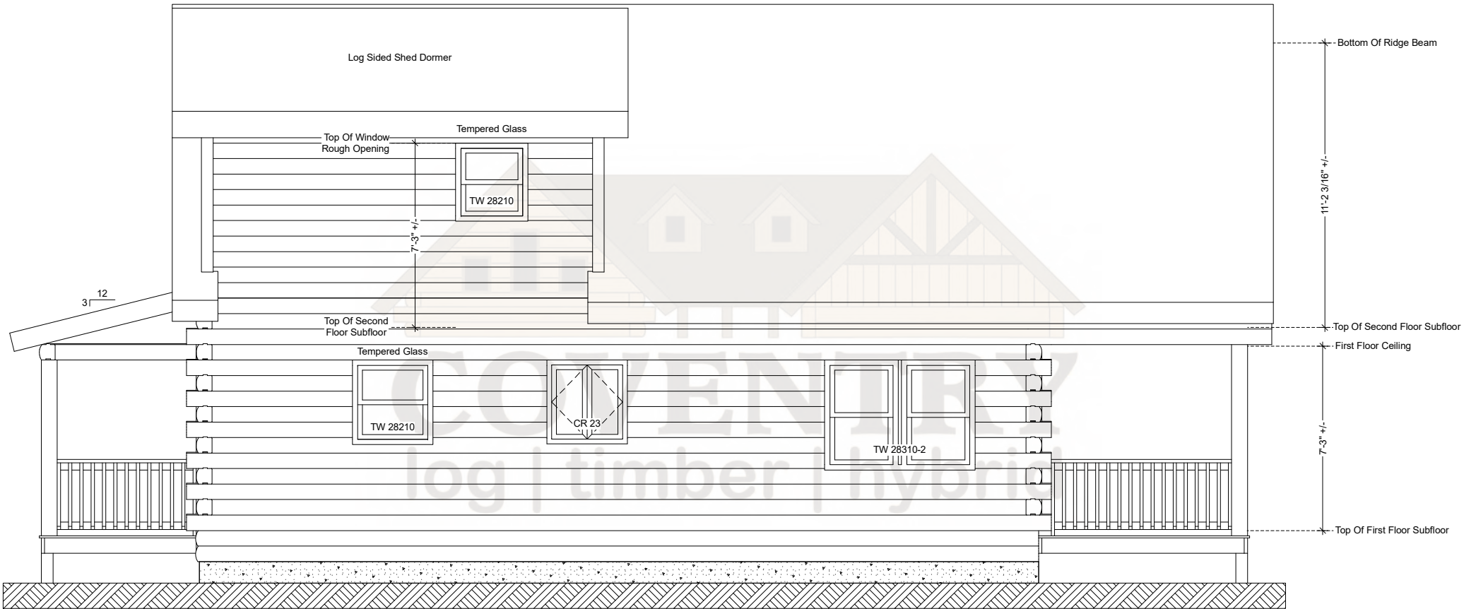
Forester Front Elevation (Shown With 8x8 D Logs)
