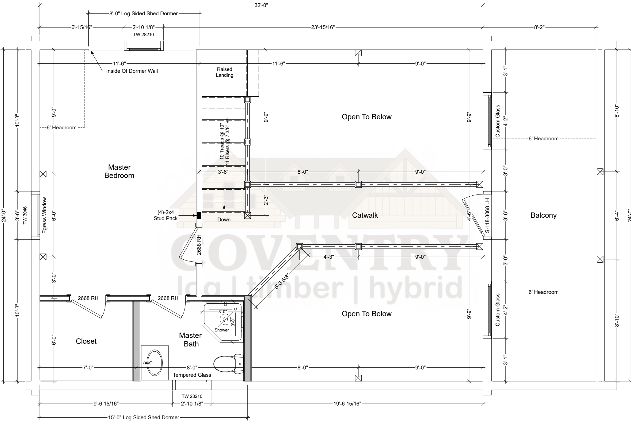
Forester Second Floor Plan (Shown With 8x8 D Logs)
