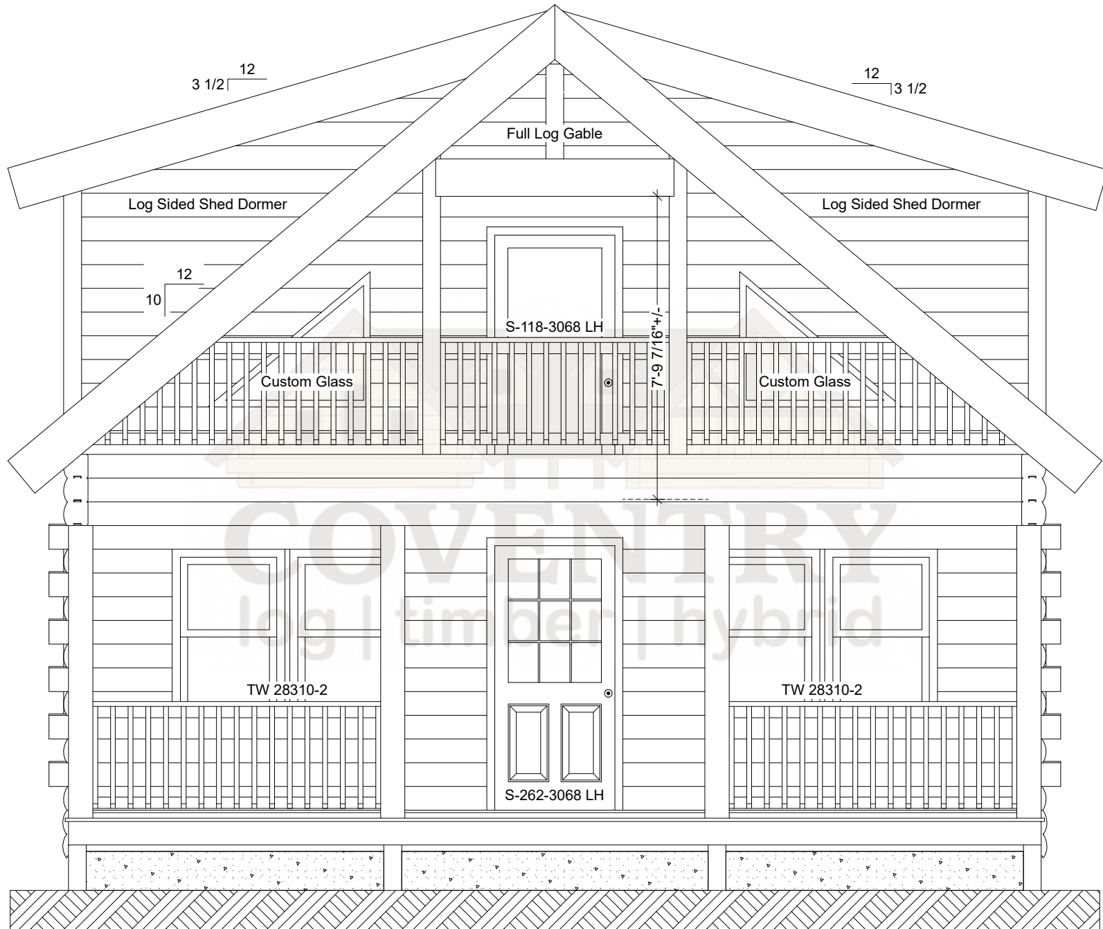
Forester Right Elevation (Shown With 8x8 D Logs)
