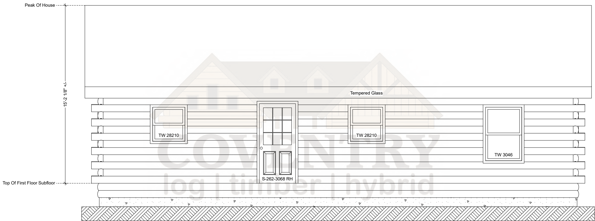
Lakeside Rear Elevation
