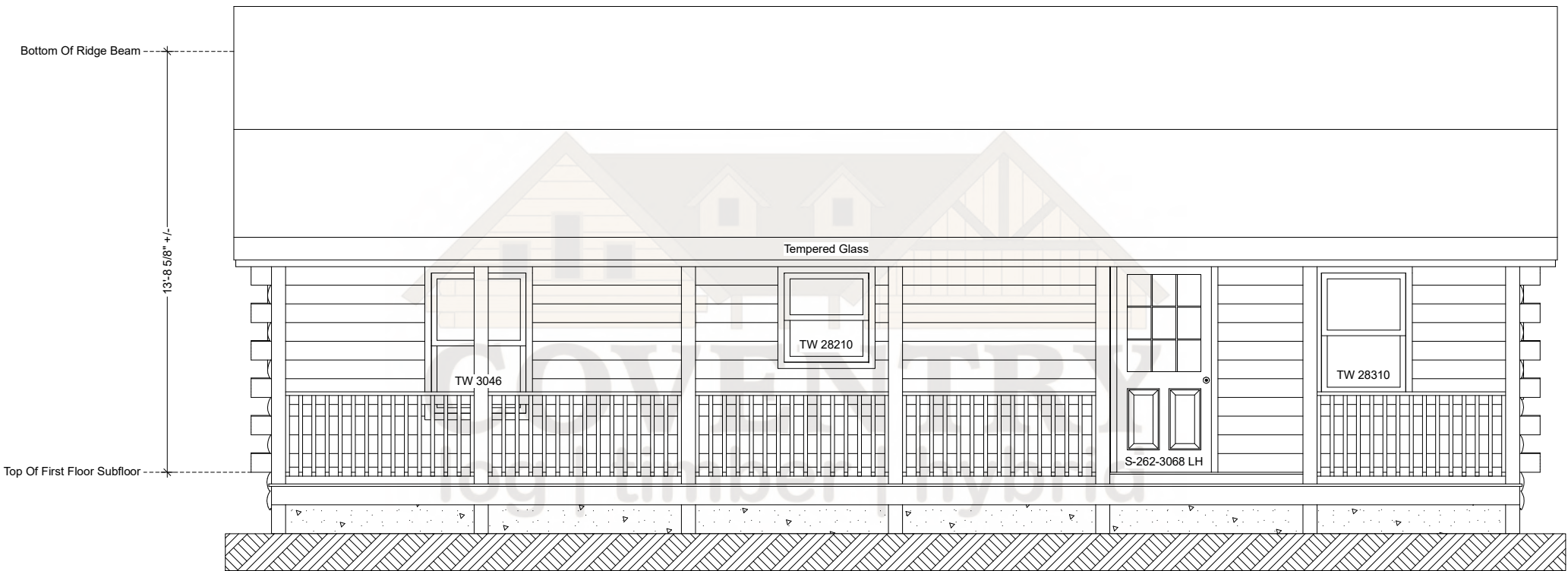
Lakeside Front Elevation
