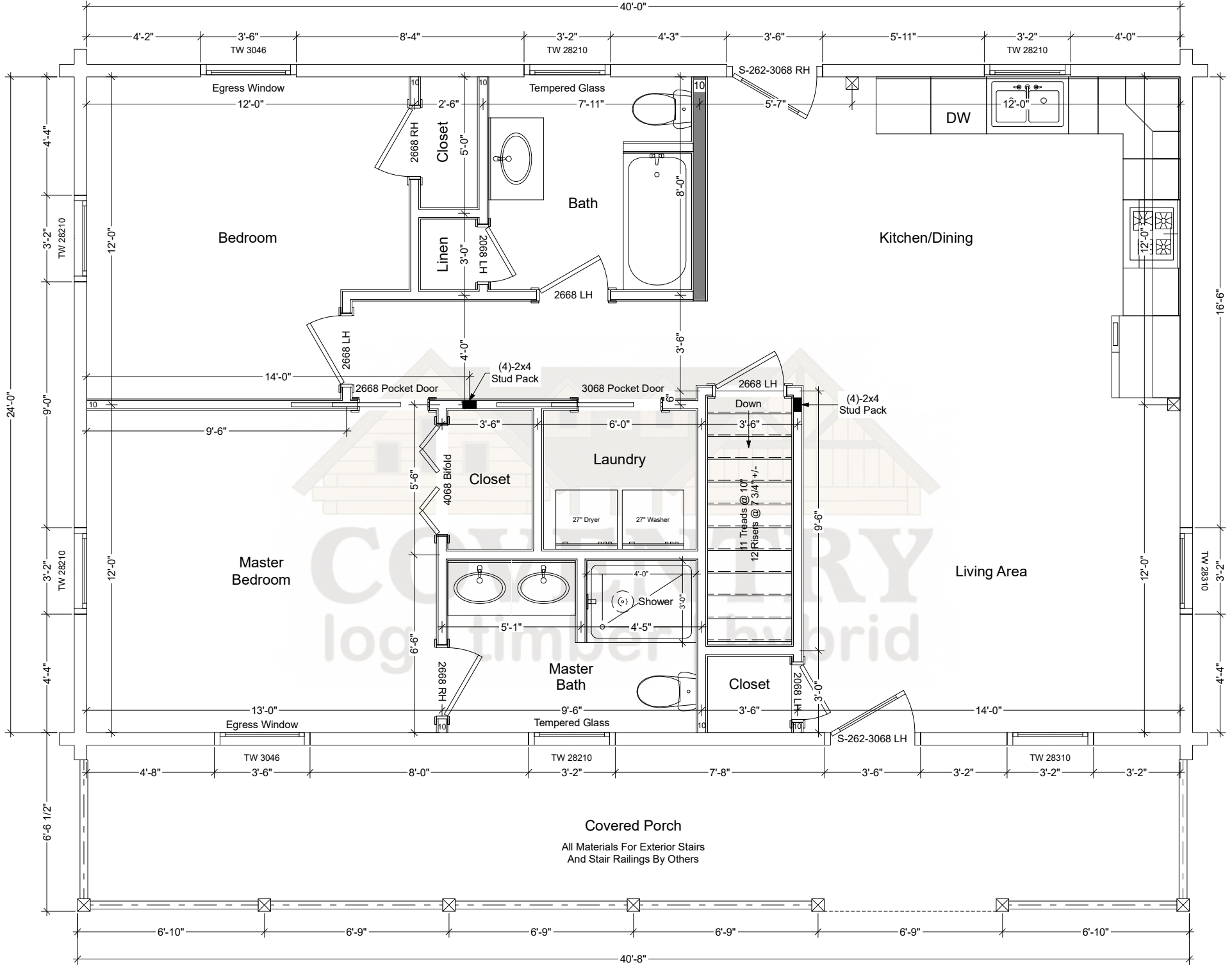
Lakeside Floor Plan
