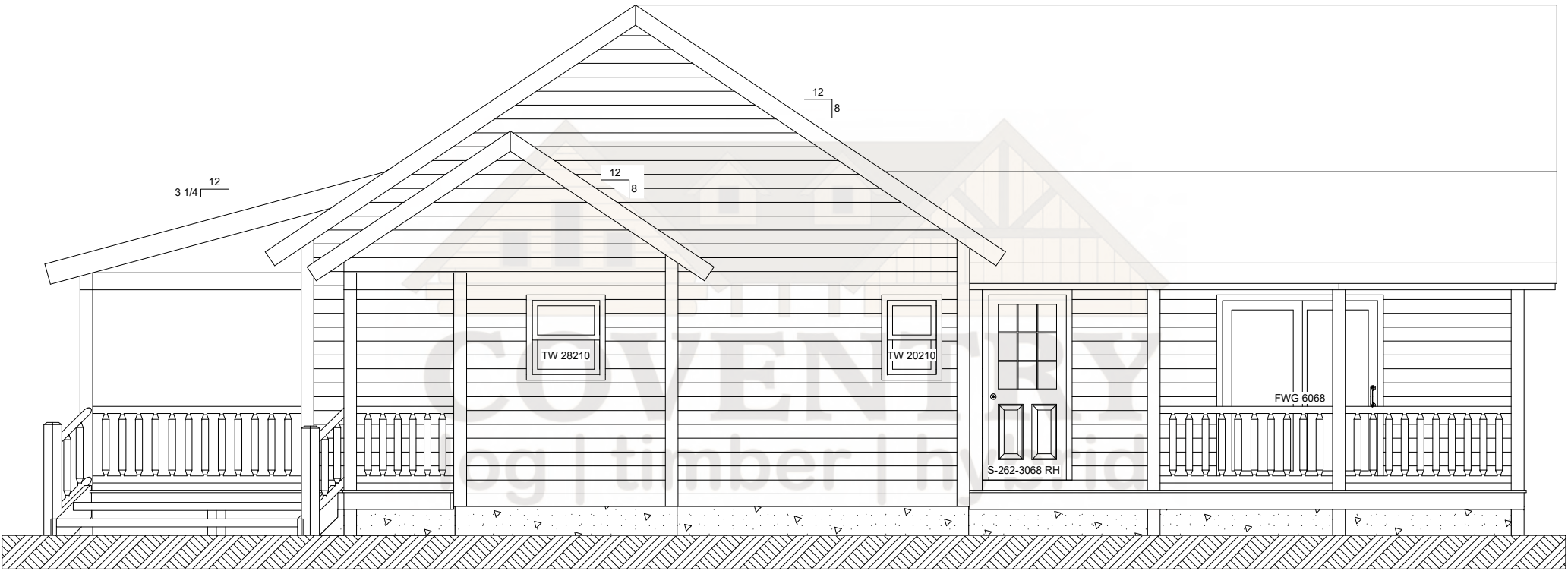
Farmhouse Right Elevation
