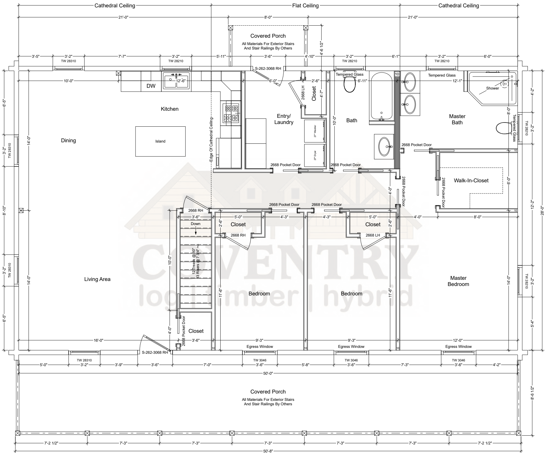
Ammonoosuc First Floor Plan
