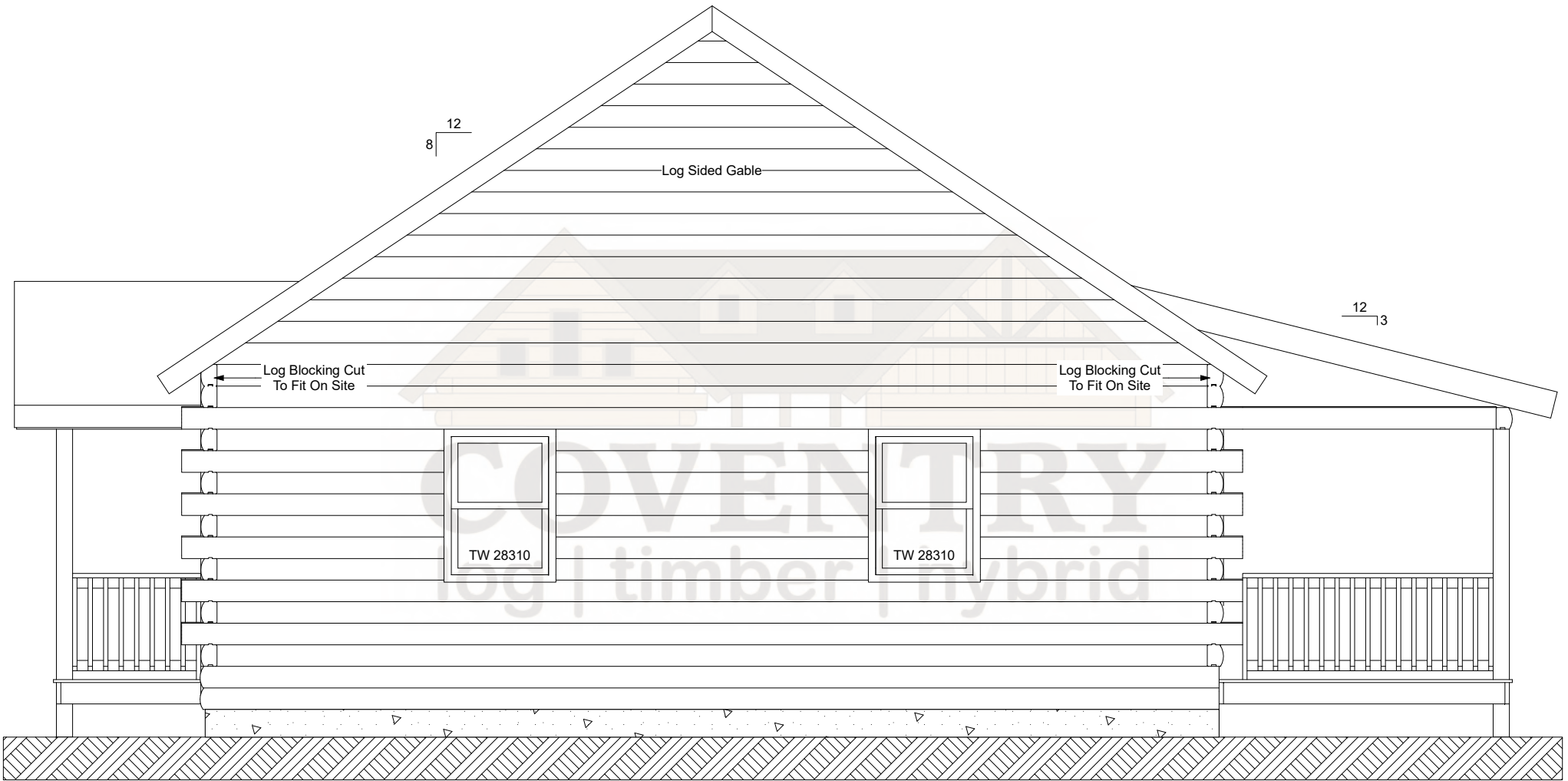
Ammonoosuc Left Elevation
