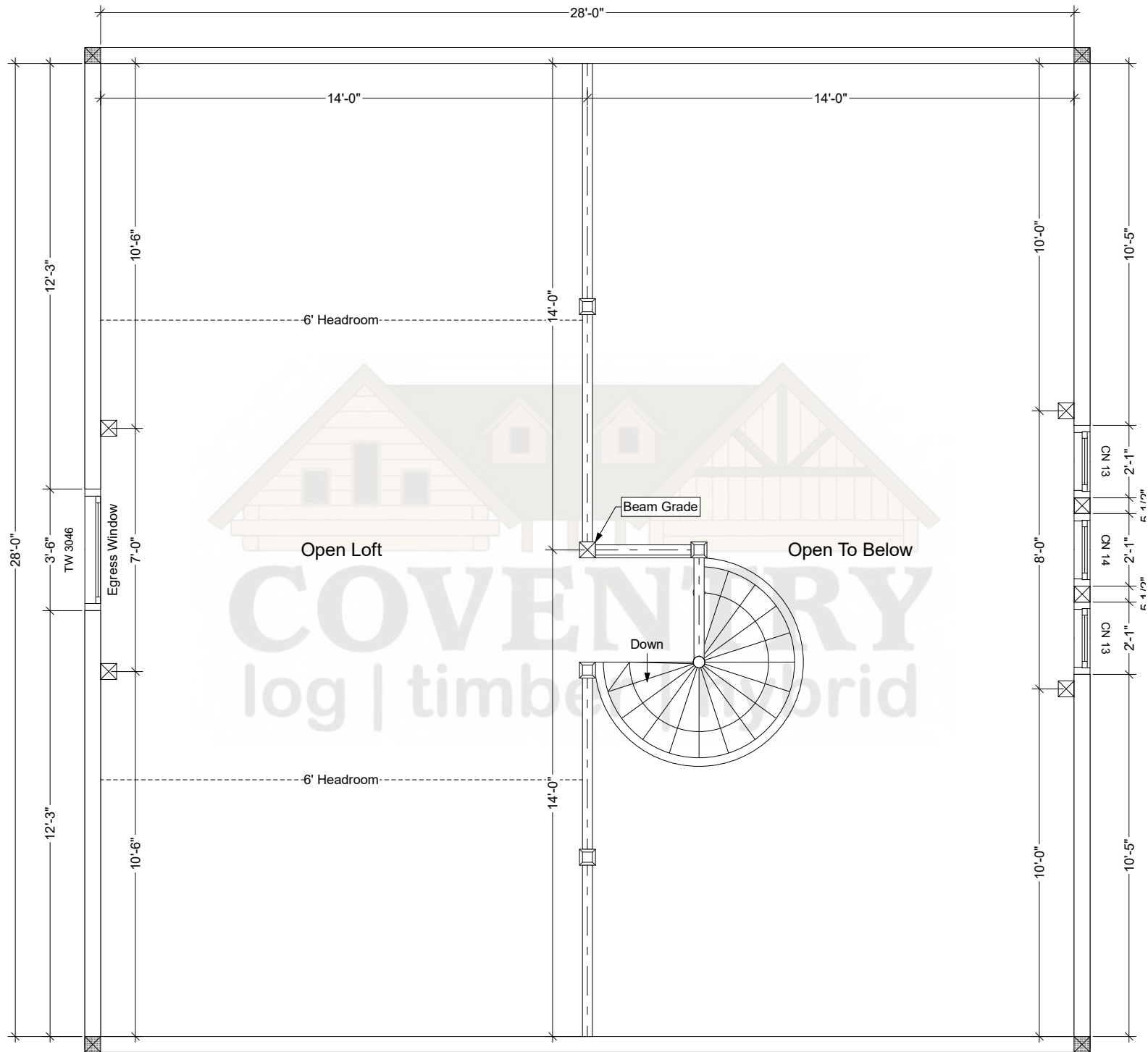
Custom Bradley Second Floor Plan
