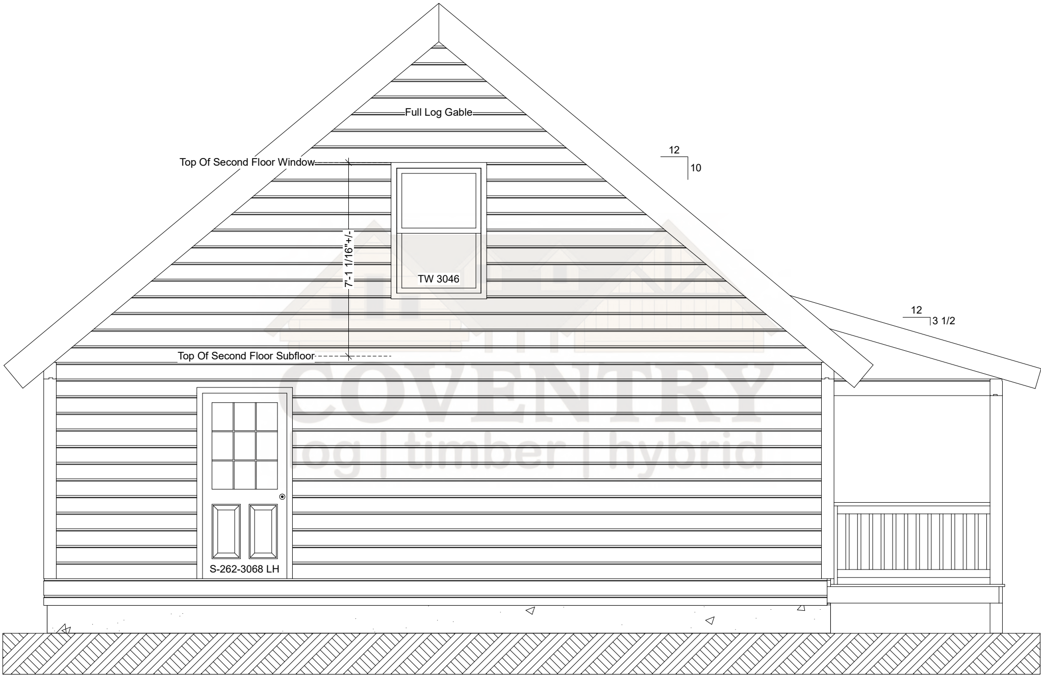
Custom Bradley Left Elevation
