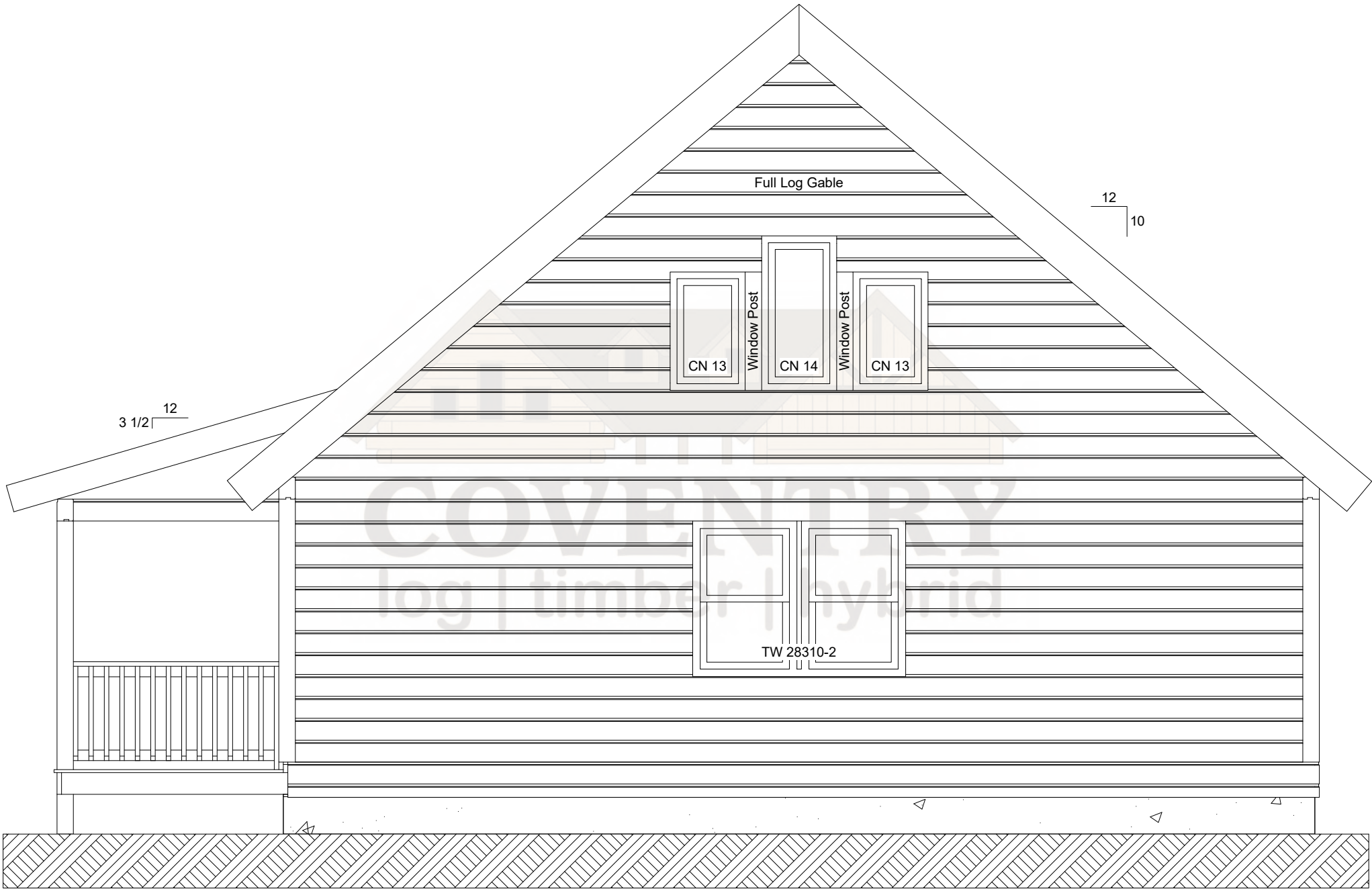
Custom Bradley Right Elevation
