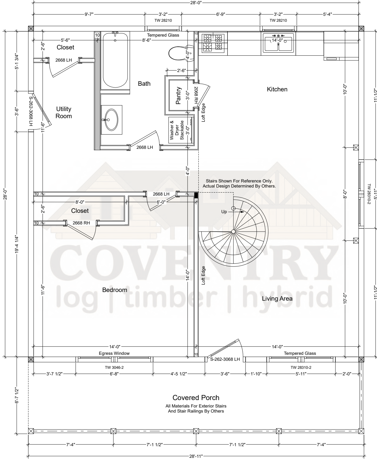
Custom Bradley First Floor Plan
