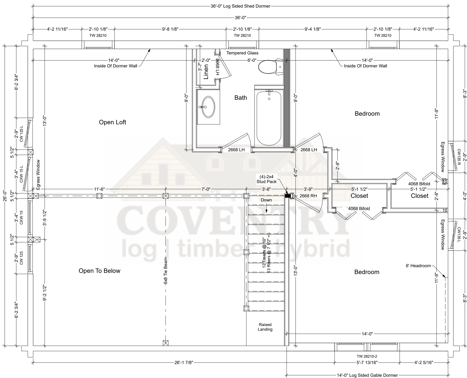
Fieldstone Second Floor Plan
