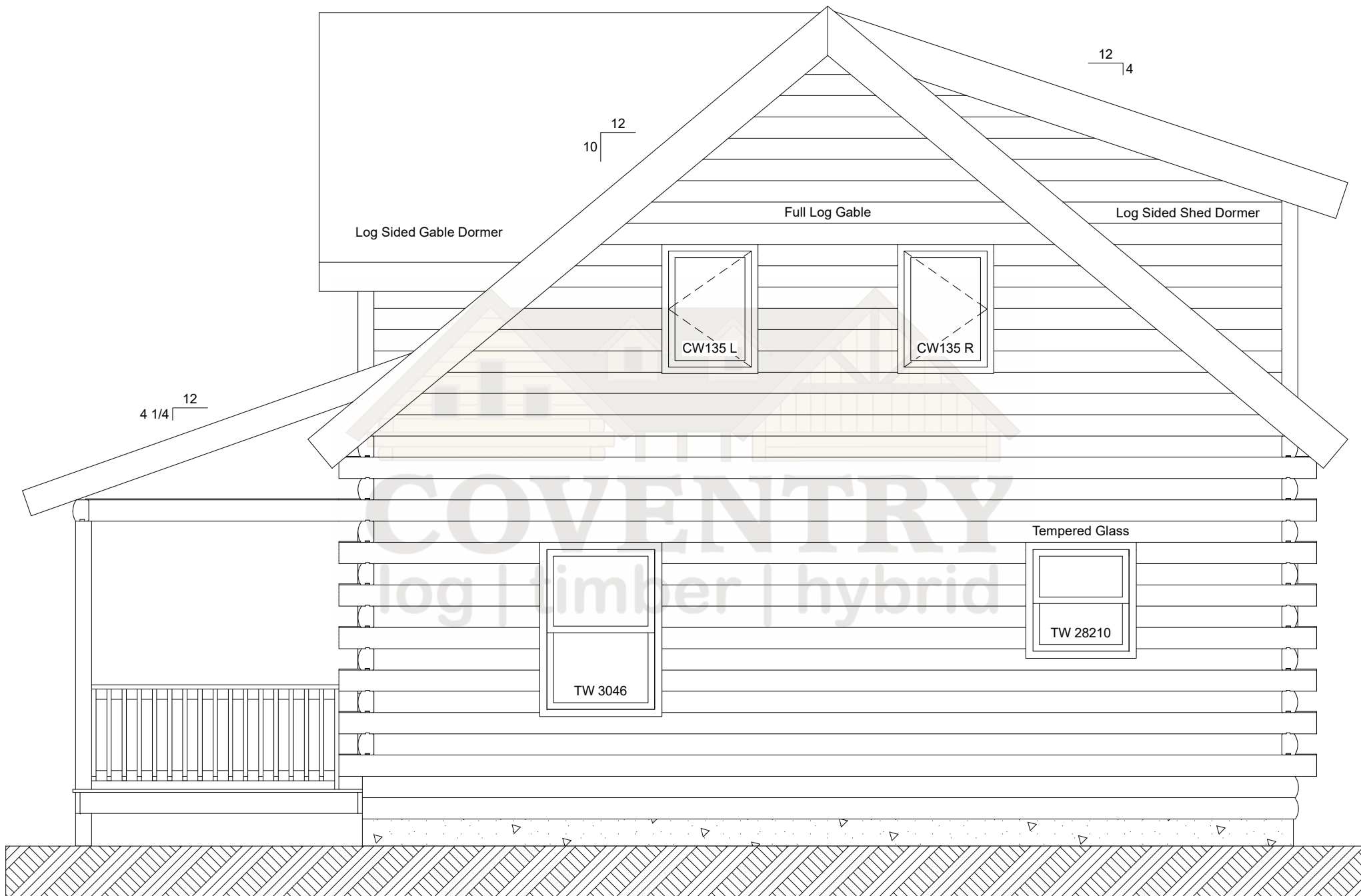
Fieldstone Right Elevation
