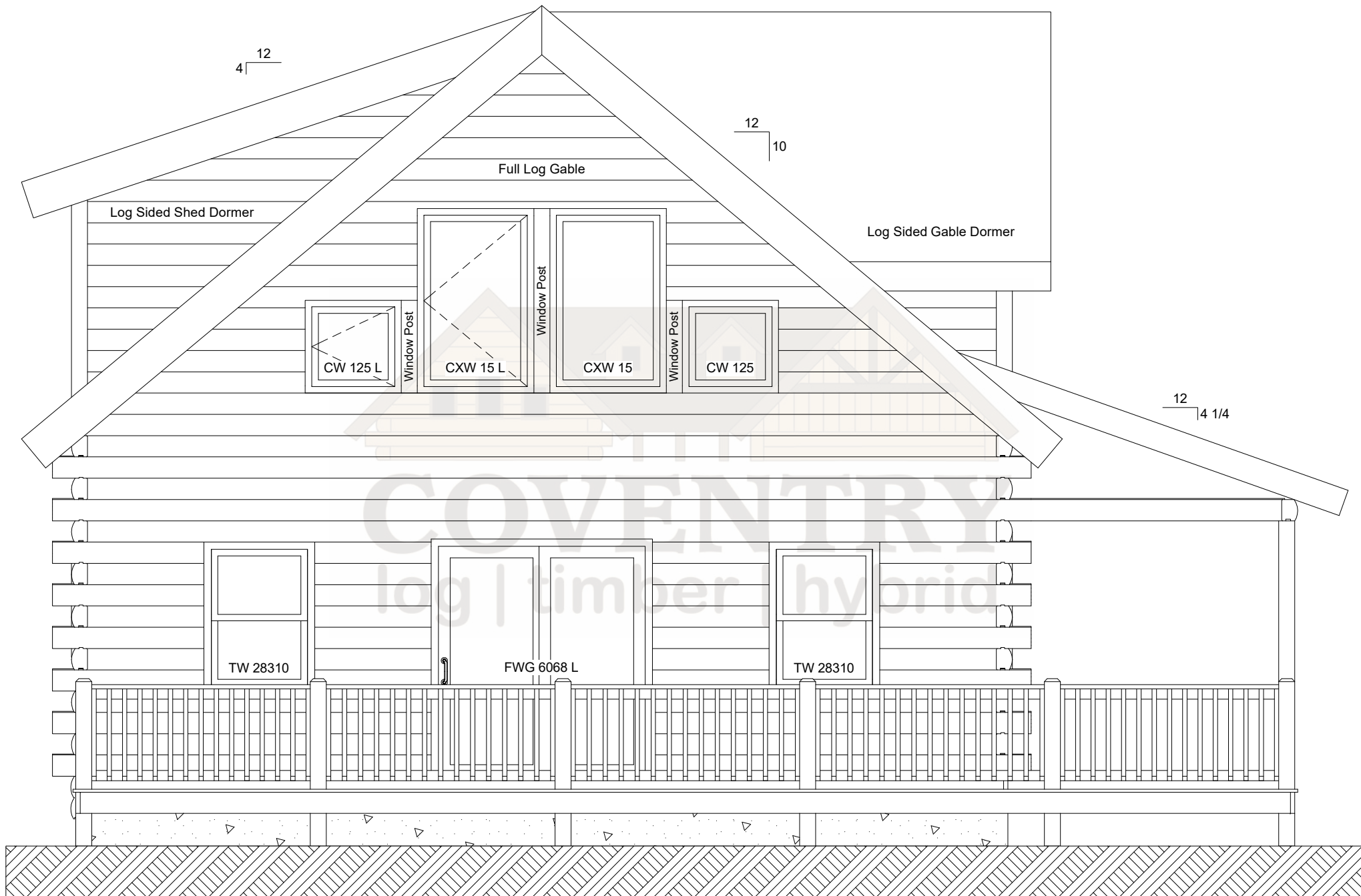
Fieldstone Left Elevation
