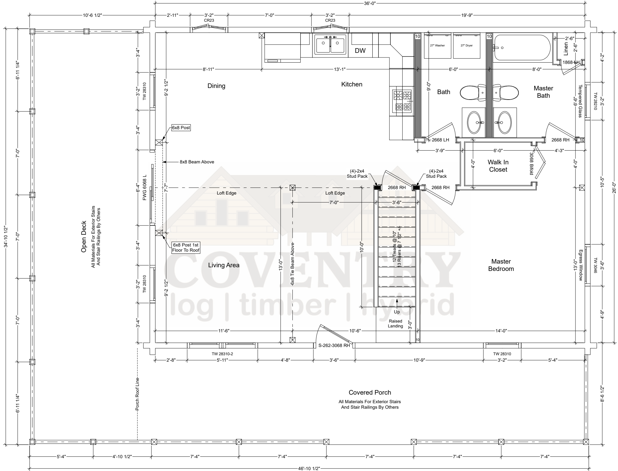
Fieldstone First Floor Plan
