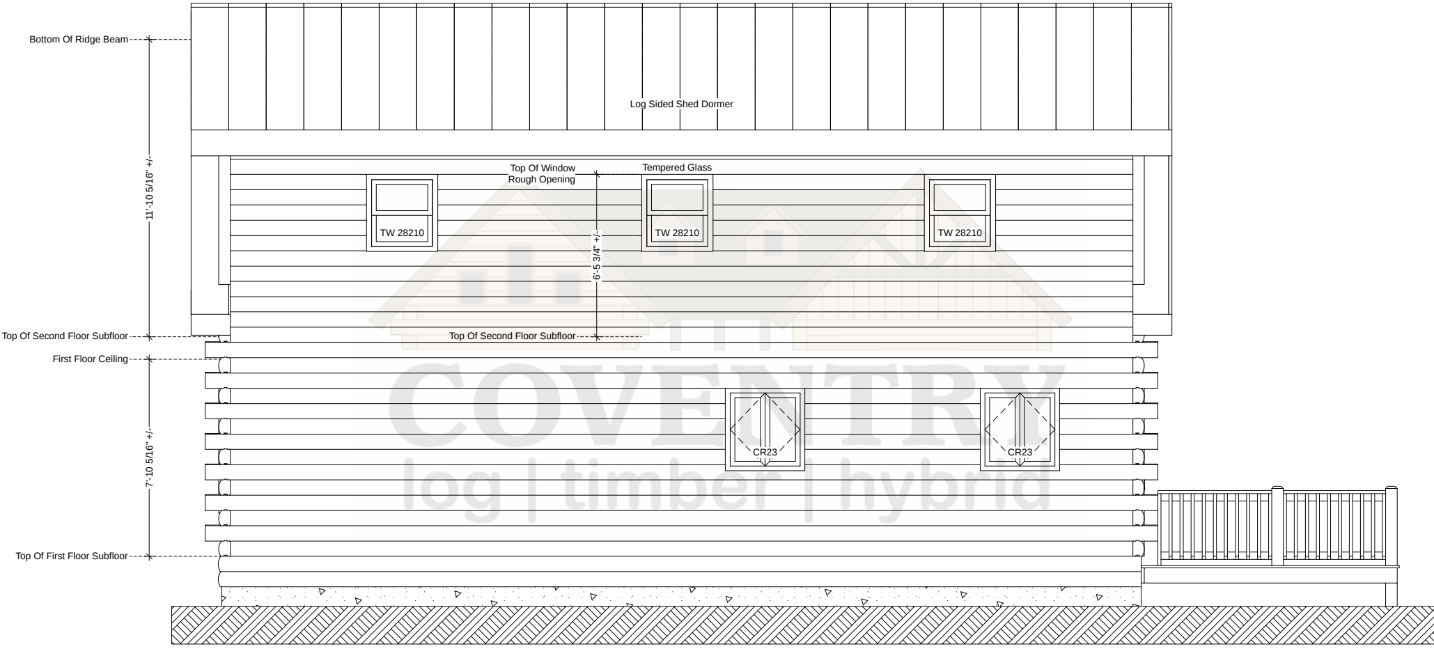
Fieldstone Rear Elevation
