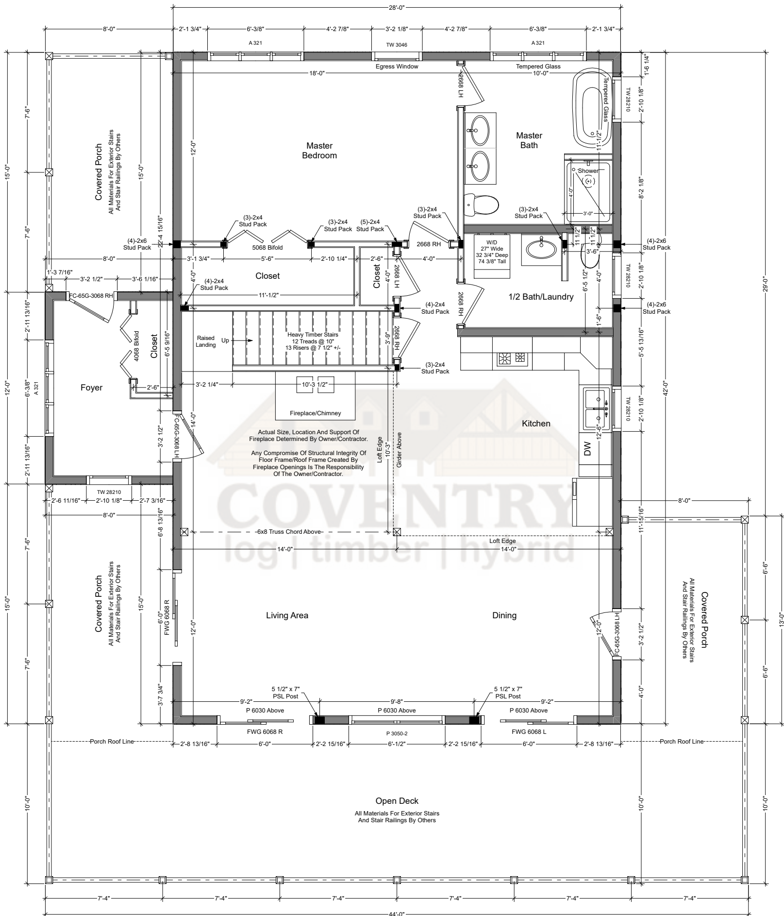
Maplewood First Floor Plan
