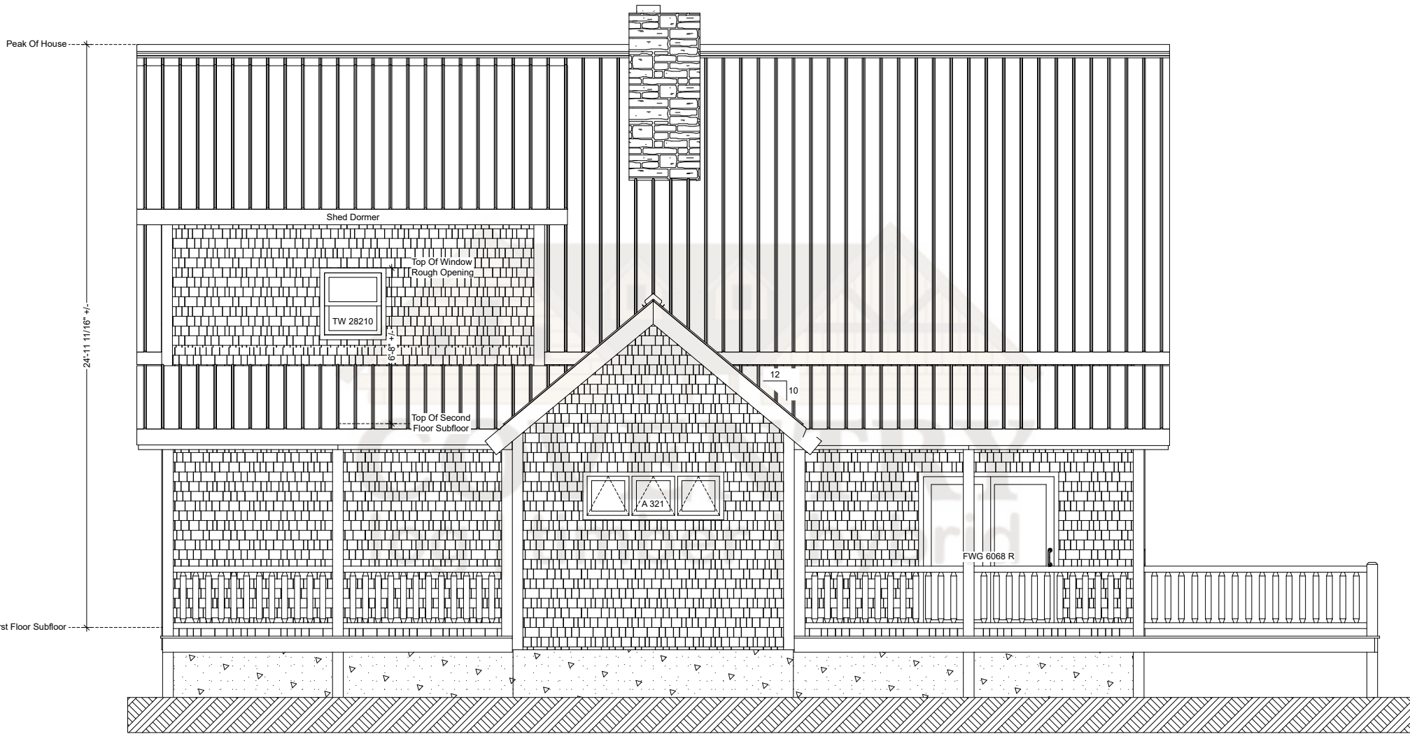
Maplewood Left Elevation
