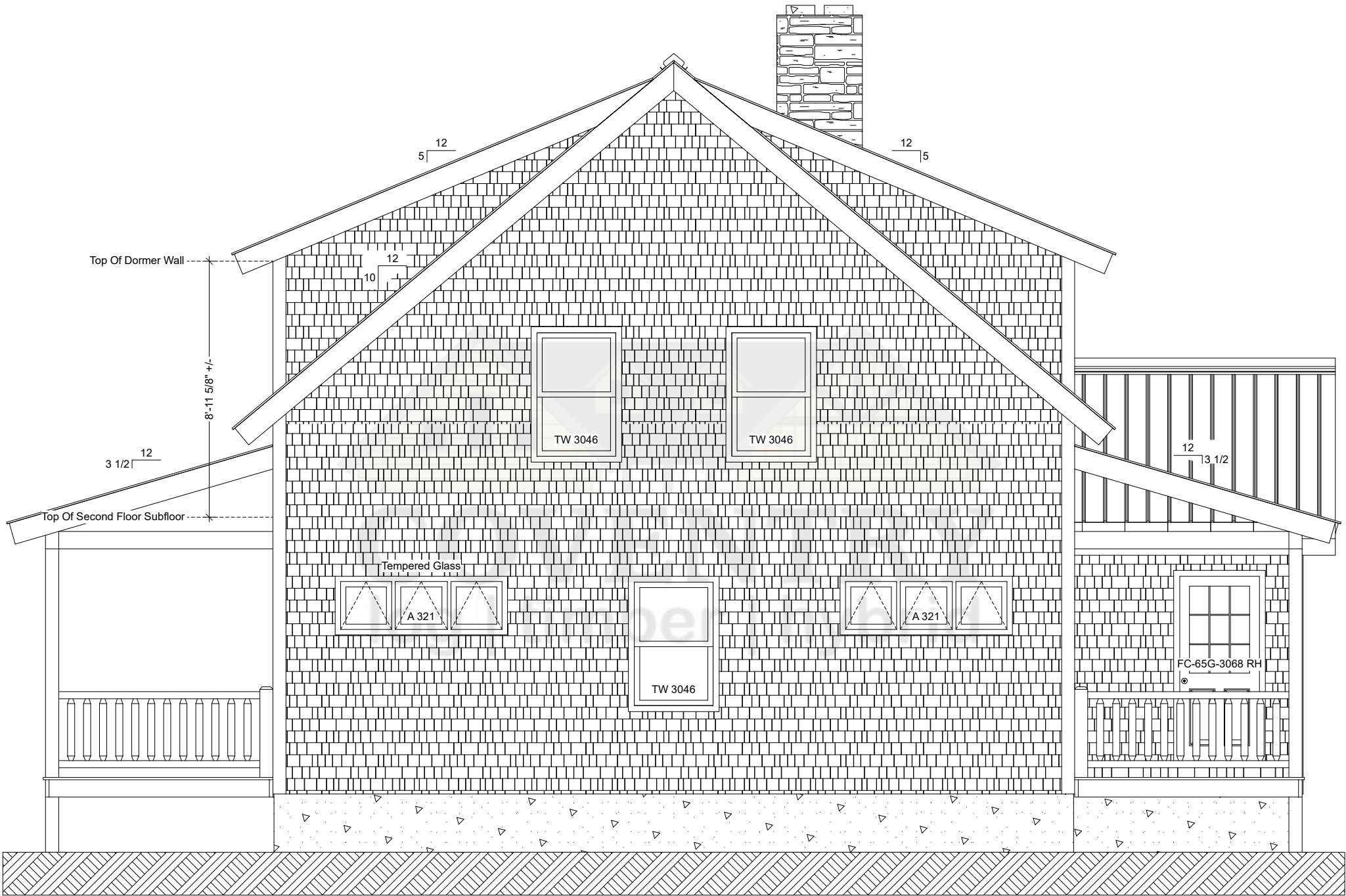
Maplewood Rear Elevation
