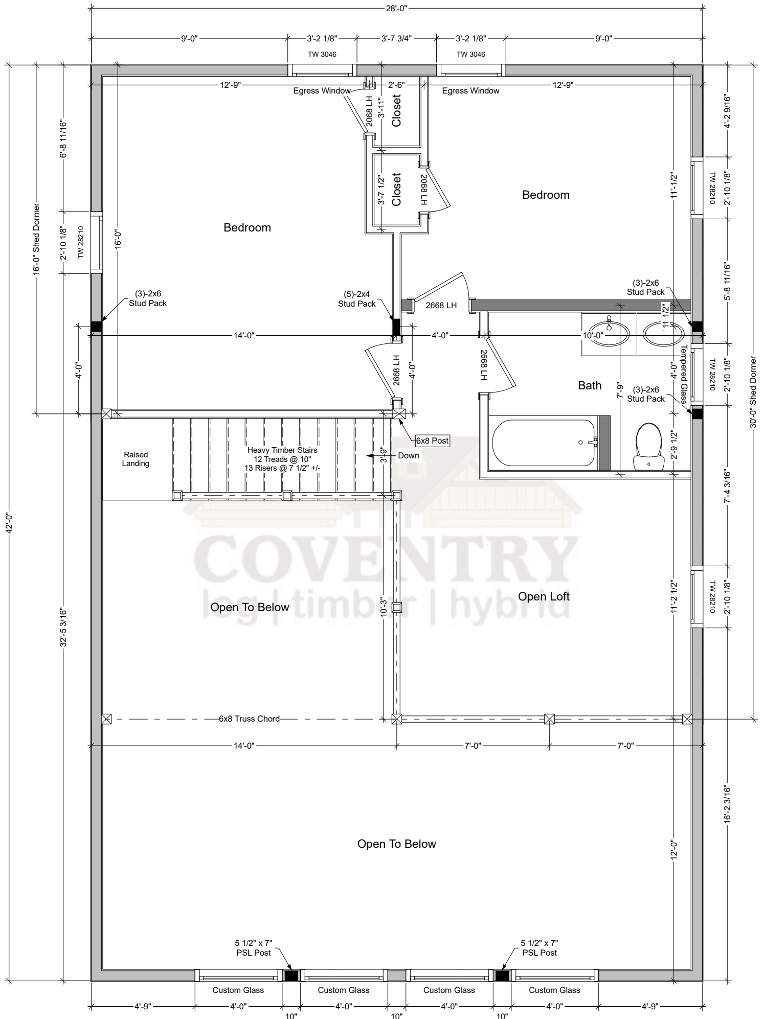
Maplewood Second Floor Plan
