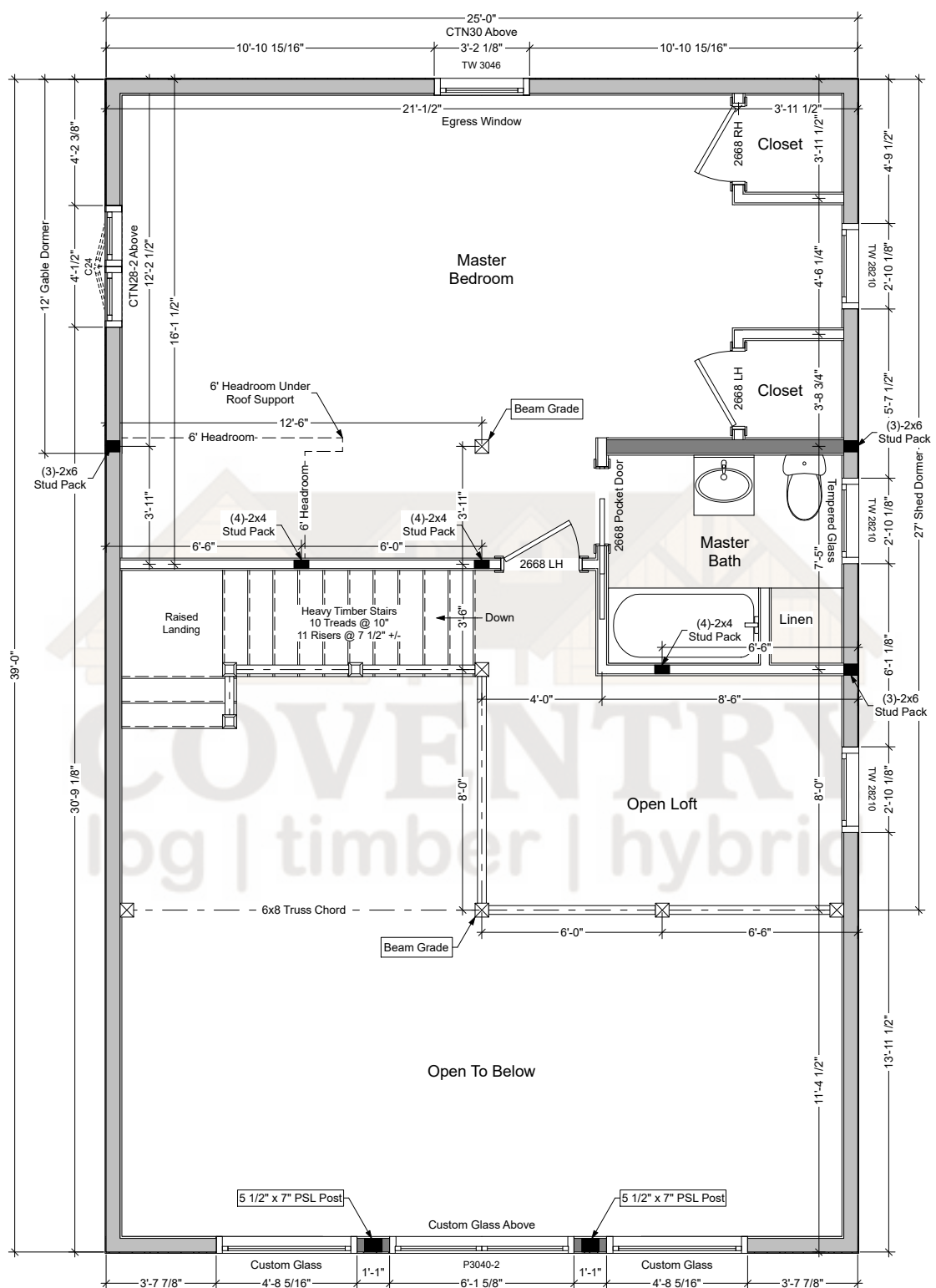
Ticonderoga Second Floor Plan
