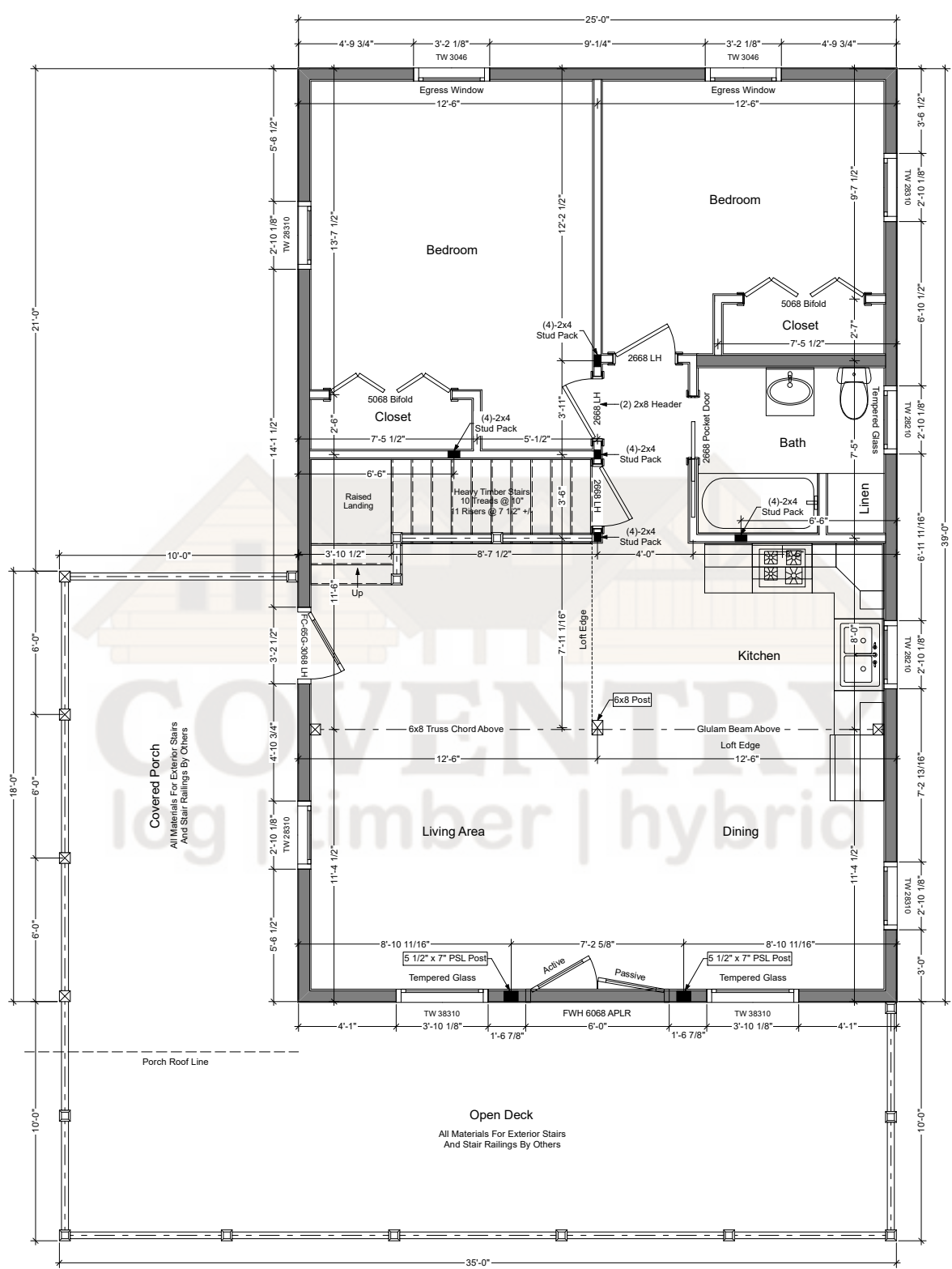
Ticonderoga First Floor Plan
