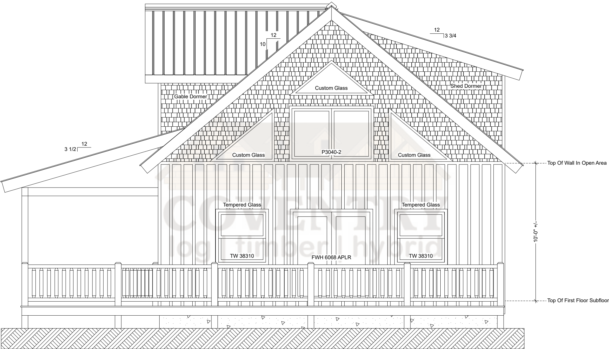
Ticonderoga Front Elevation
