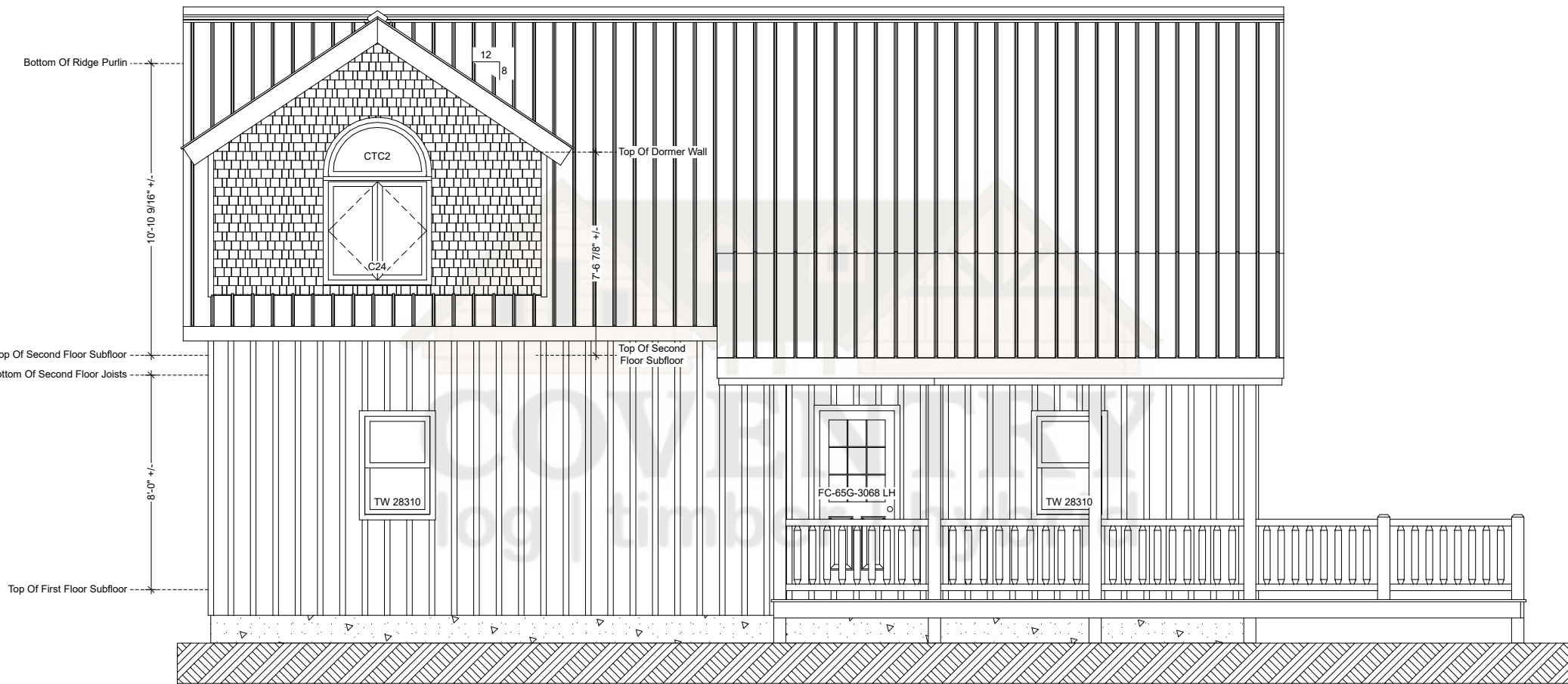
Ticonderoga Left Elevation
