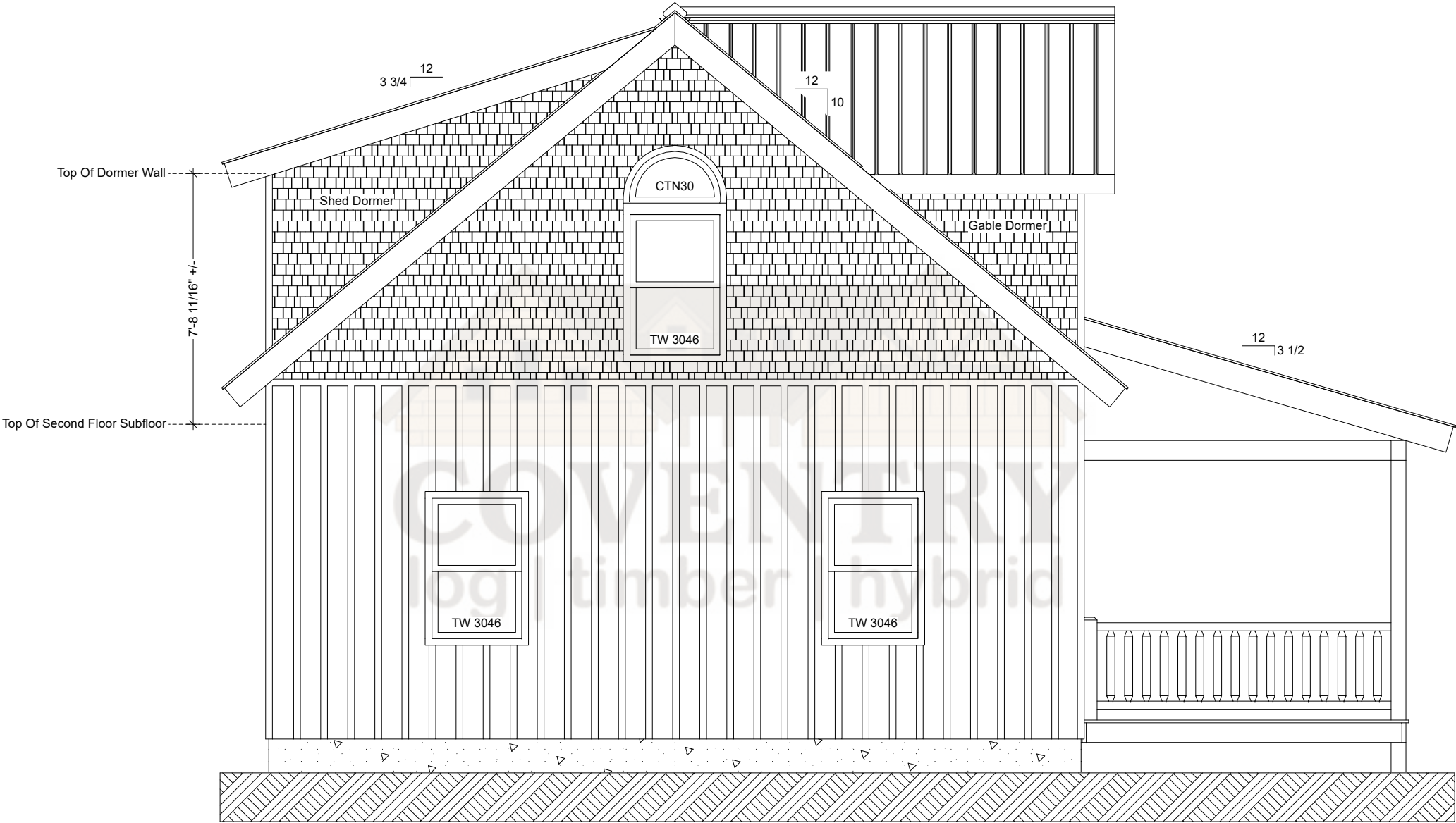
Ticonderoga Rear Elevation
