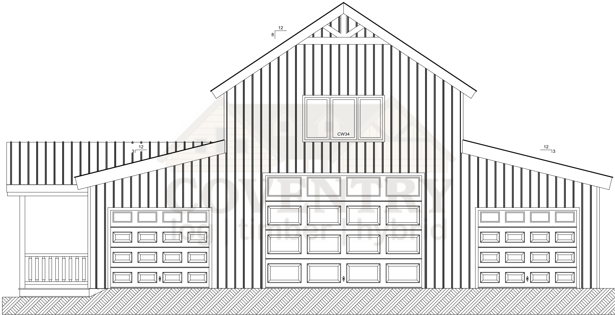
Yellowstone Rear Elevation
