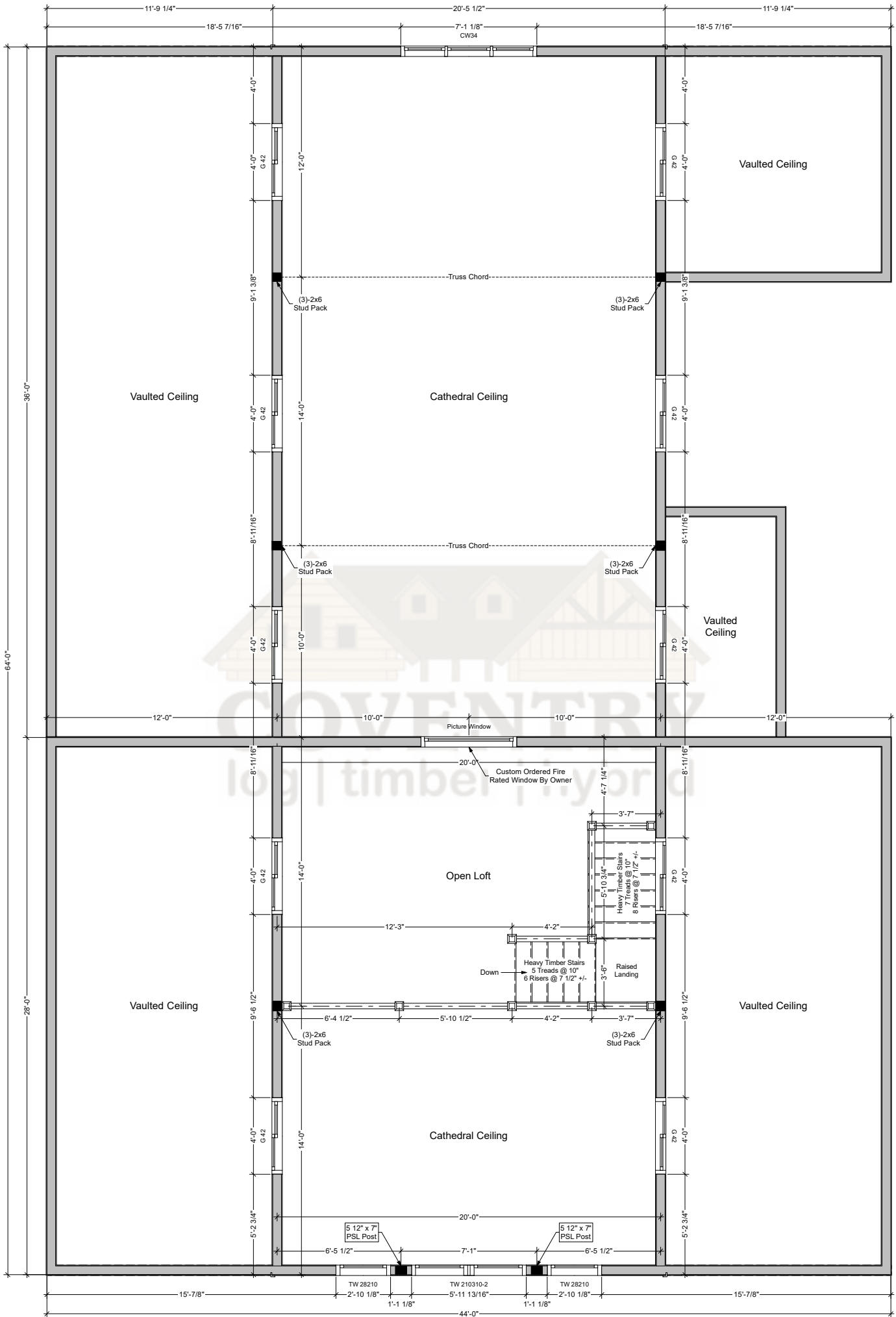
Yellowstone Second Floor Plan
