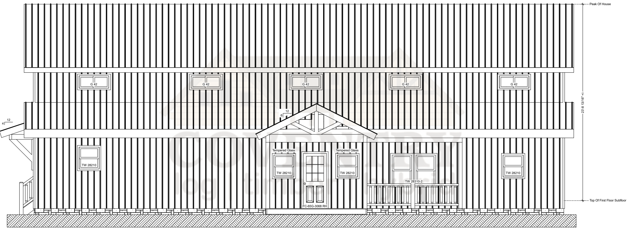
Yellowstone Right Elevation
