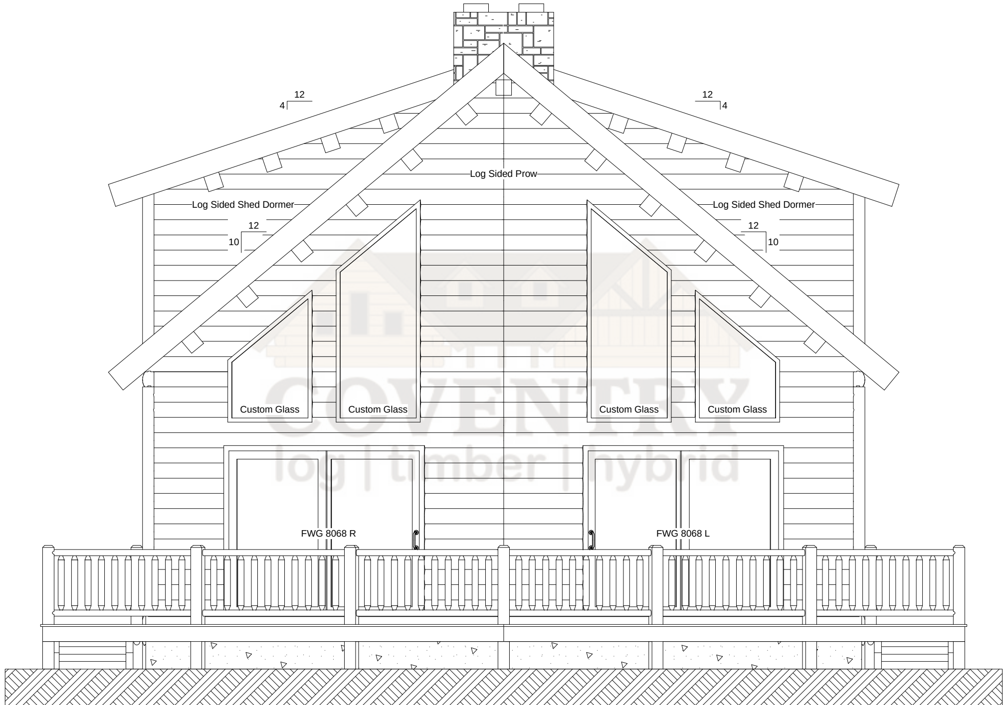
Ridgeview Left Elevation
