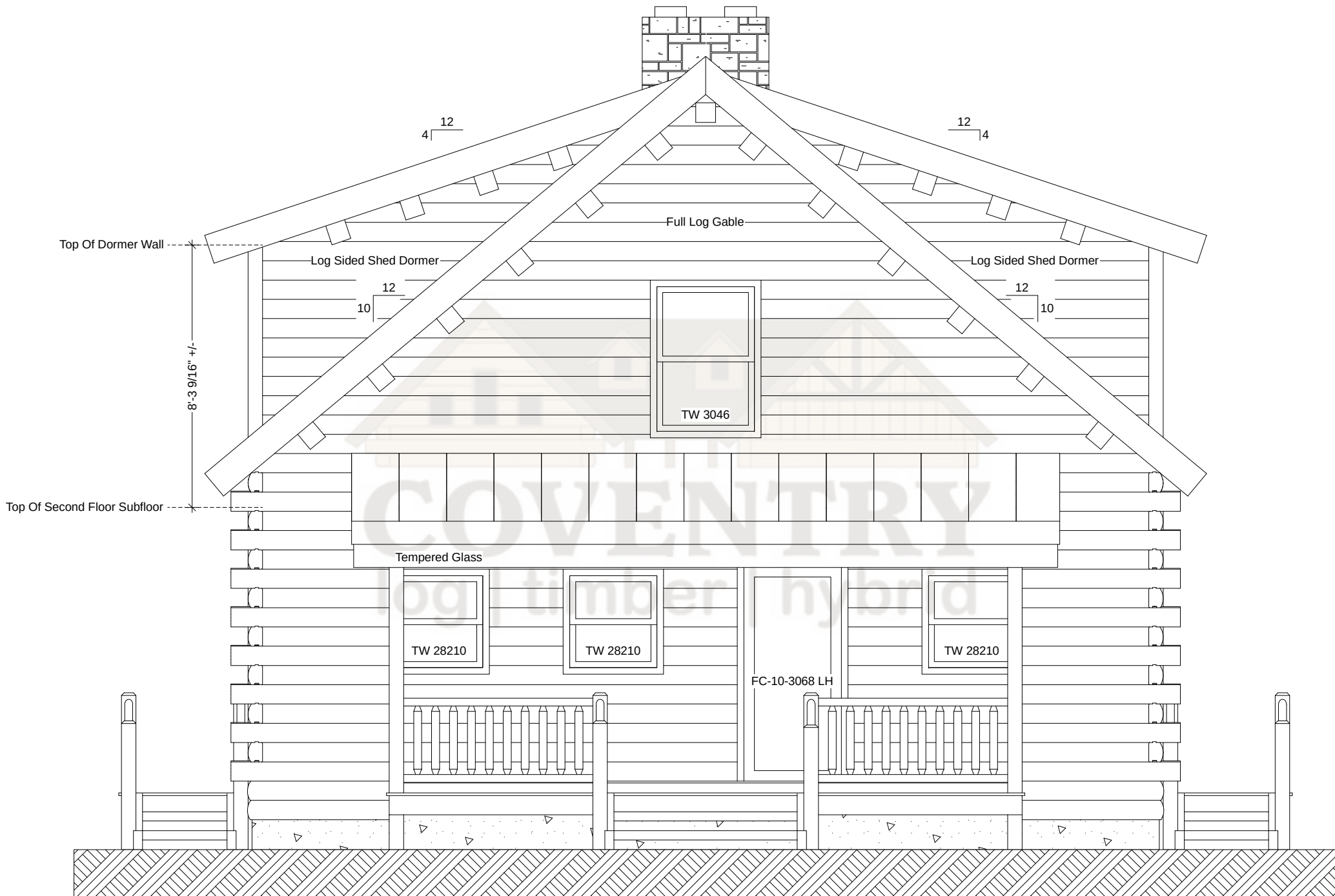
Ridgeview Right Elevation
