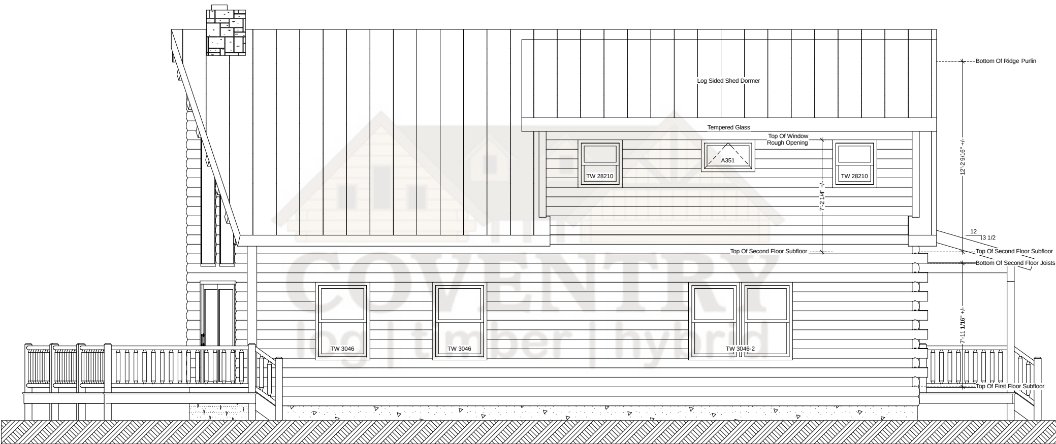
Ridgeview Front Elevation
